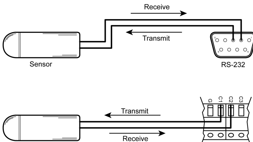
FIGURE 25: Use of RS-232 and Digital I/O when Reading RS-232 Devices
