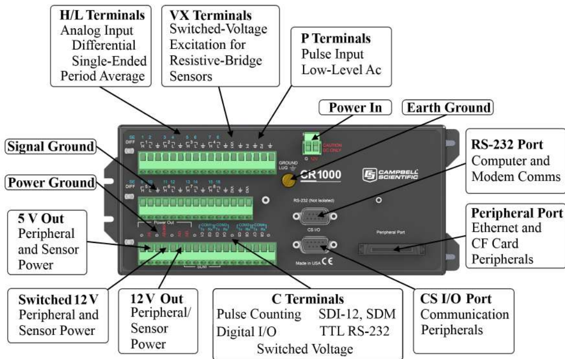
FIGURE 1: Wiring Panel
