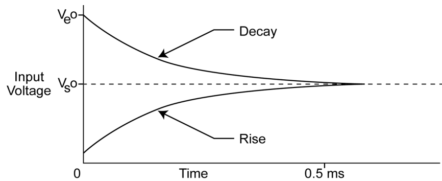
FIGURE 86: Input voltage rise and transient decay
