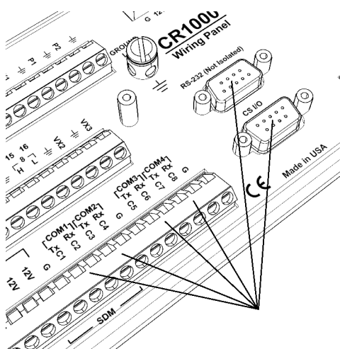
FIGURE 25: Use of RS-232 and Digital I/O when Reading RS-232 Devices
