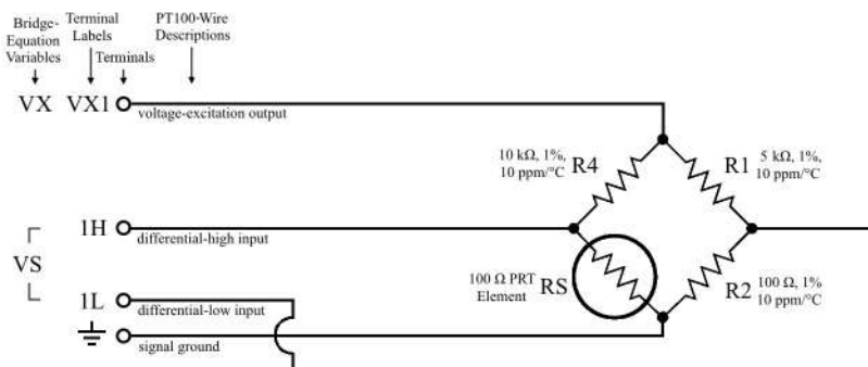
FIGURE 67: PT100 BrFull() Four-Wire Full-Bridge Schematic
