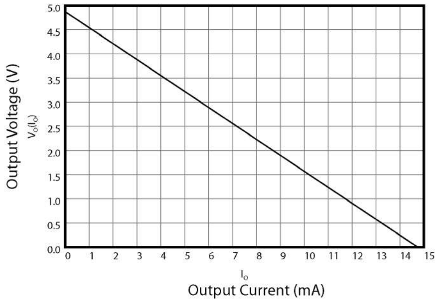
FIGURE 97: Current sourcing from C terminals configured for control
