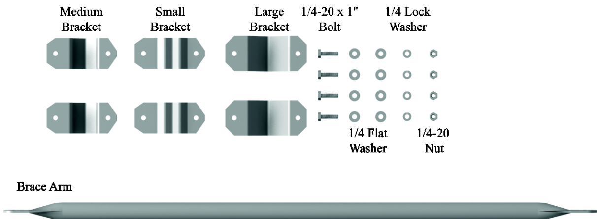
FIGURE 6-5. CMB200 components
