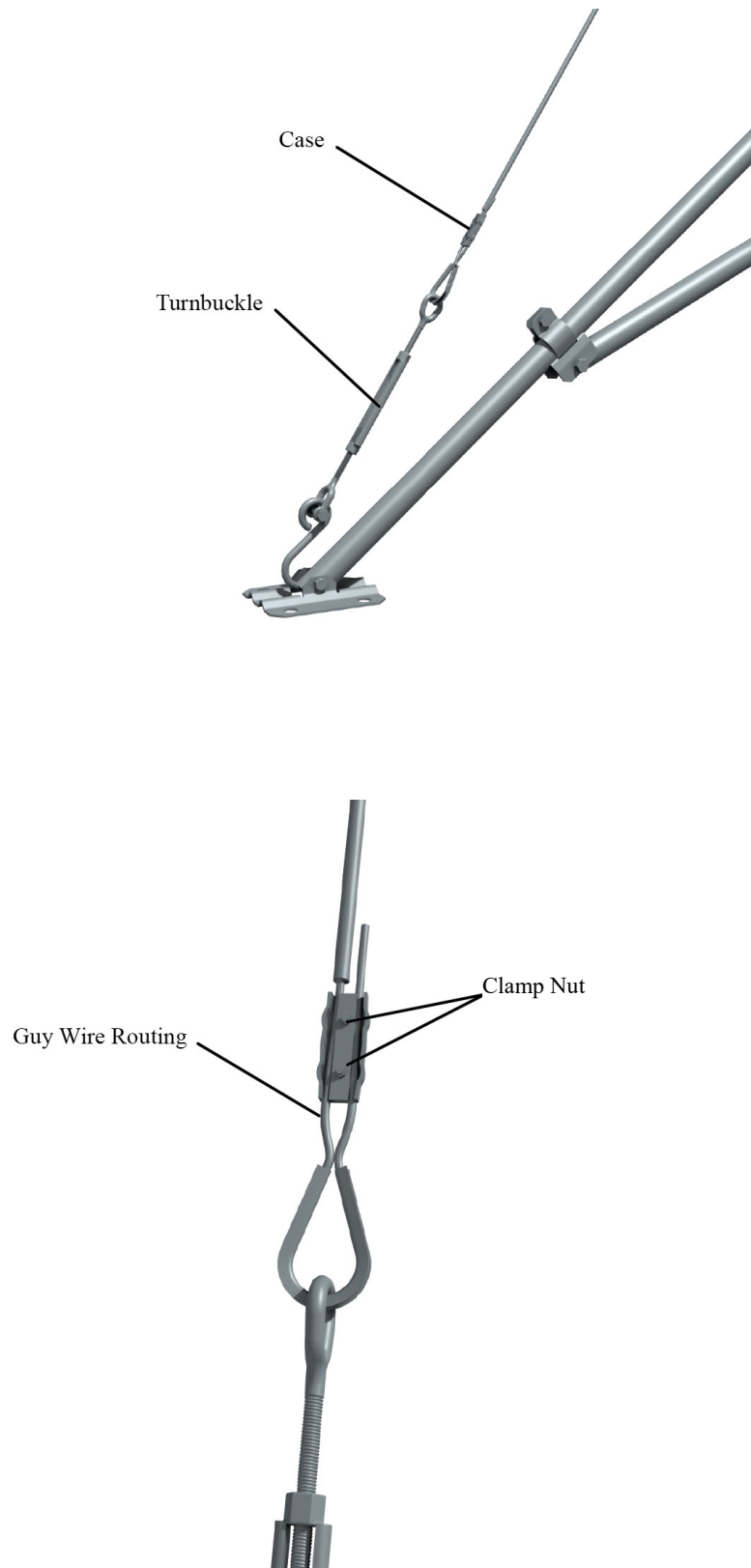
FIGURE 5-4. Leg attachment
