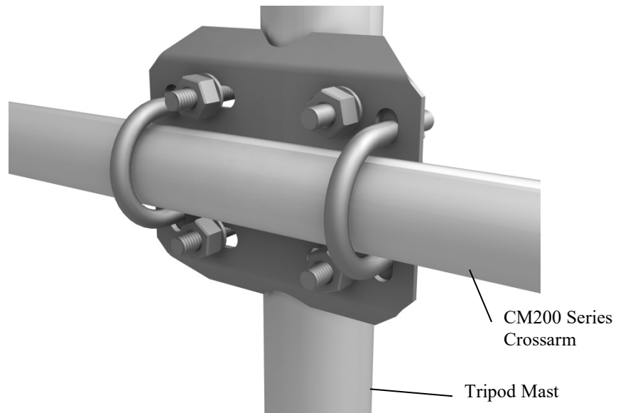
FIGURE 5-9. CM204 Crossarm
