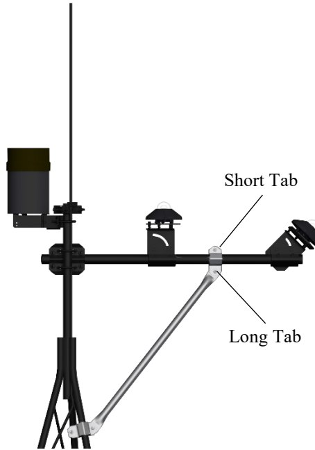
FIGURE 6-4. CMB200 Crossarm Brace Kit
