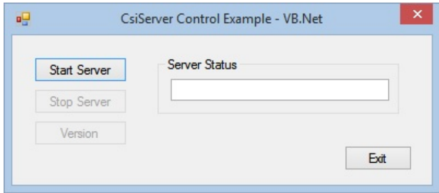
FIGURE 3-1. CsiServer Example
