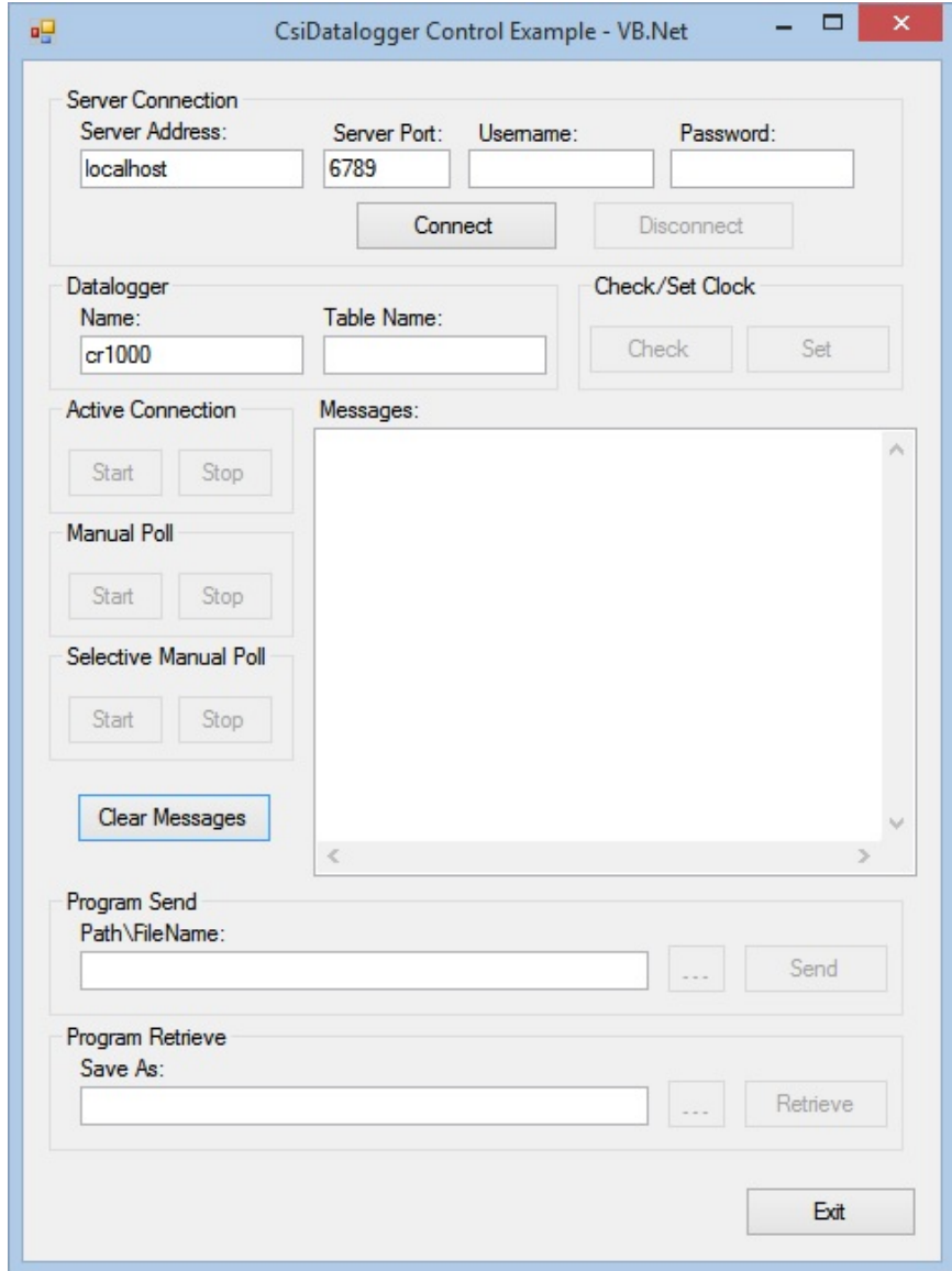
FIGURE 9-1. CsiDatalogger Example
