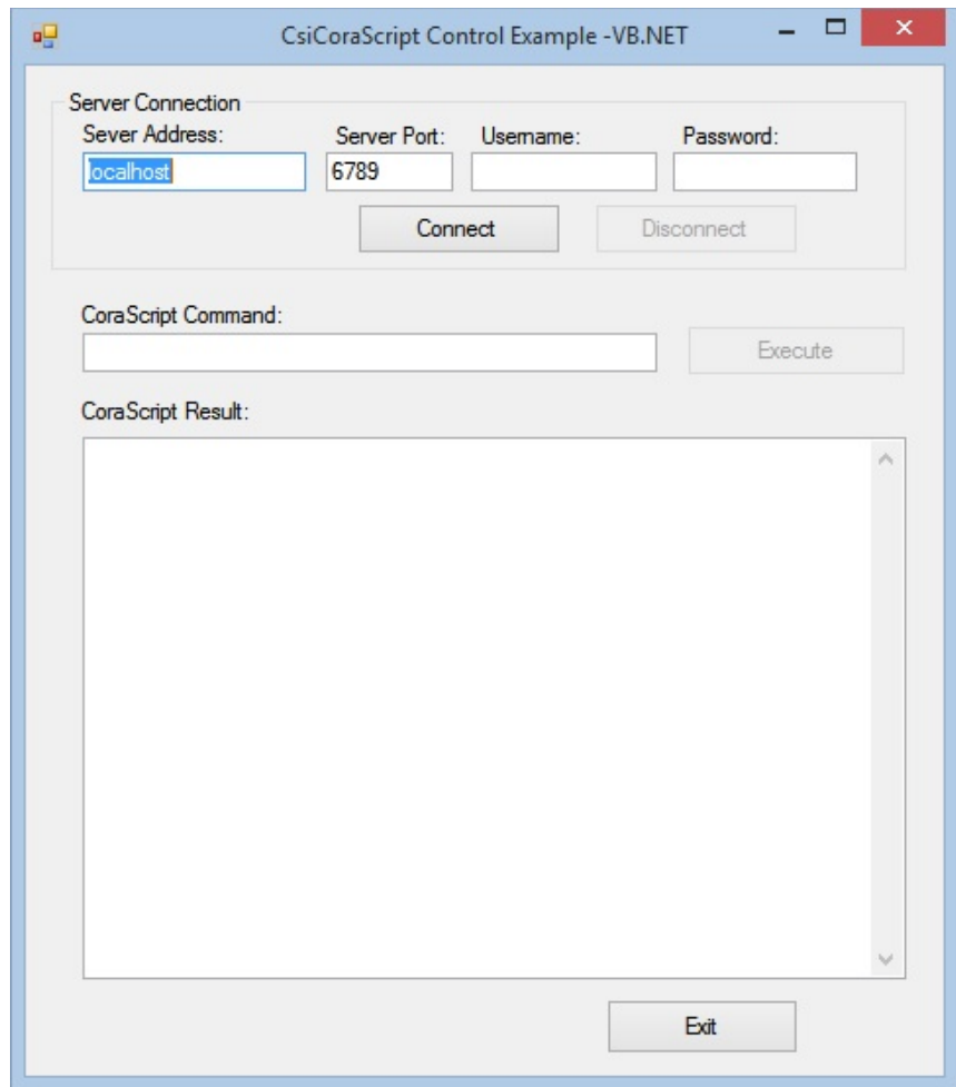
FIGURE 5-1. CsiCoraScript Example
