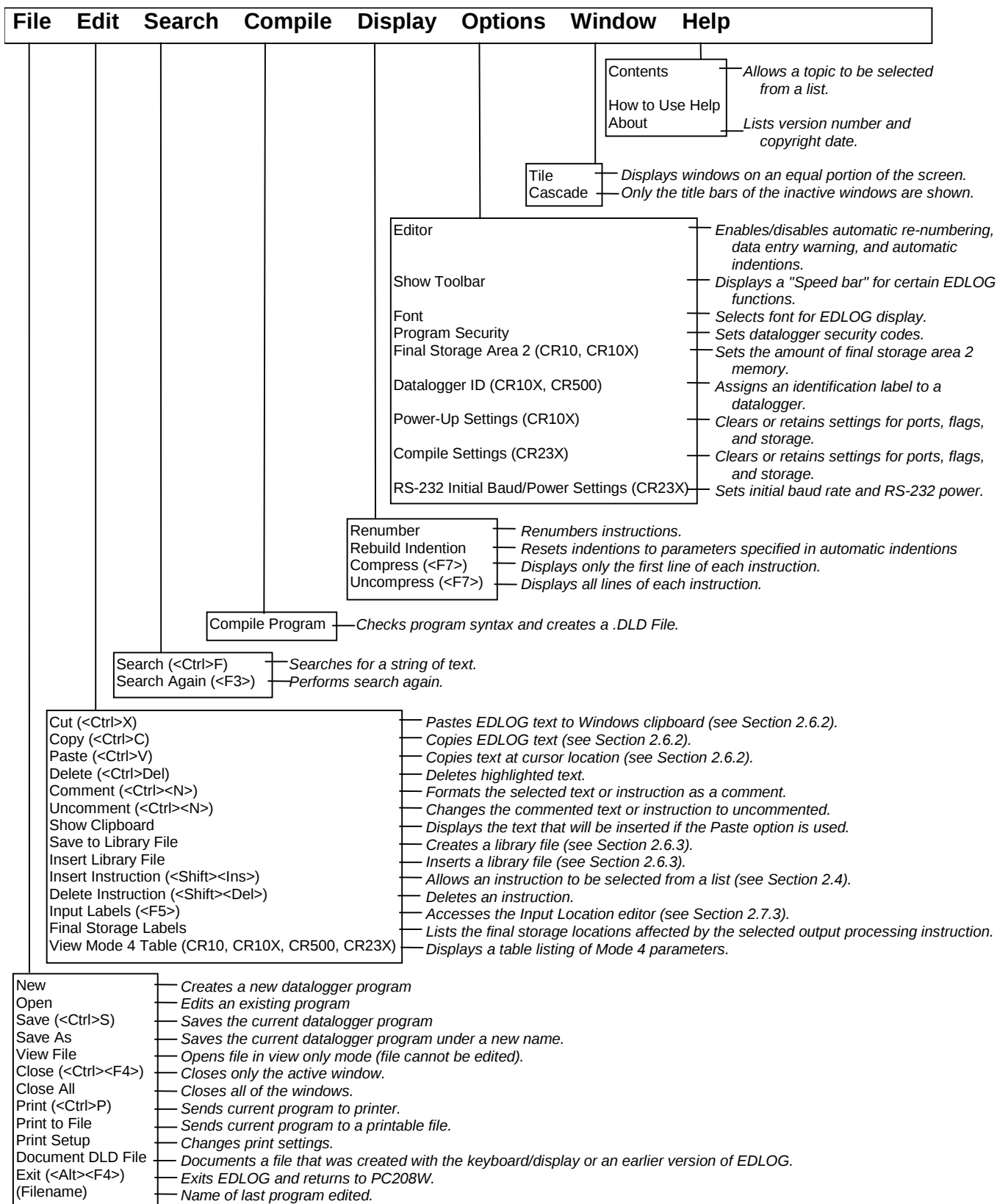
FIGURE 2.1-1. EDLOG Menu
