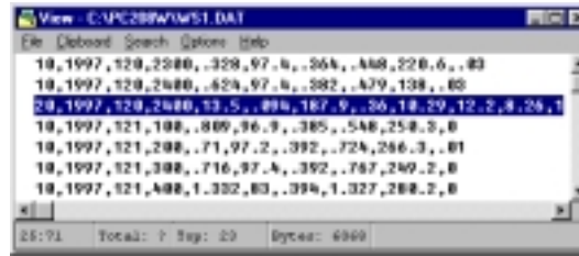
FIGURE 3.2-1. Data File
