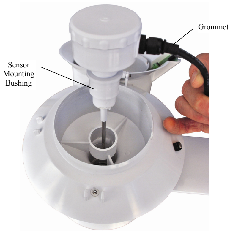
FIGURE B-1. 43347 Probe and Bushing
