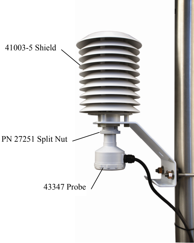
FIGURE 3-3. 41003-5 Radiation Shield Mounted to Tripod Mast
