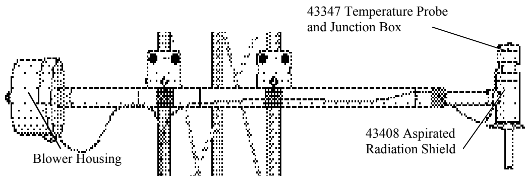
FIGURE C.1-1. 43347 RTD Temperature Probe and 43408 Aspirated Radiation Shield
