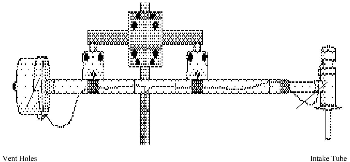
FIGURE C.2-1. PN 7515 10 m Aspirated Shield Mounting Bracket
