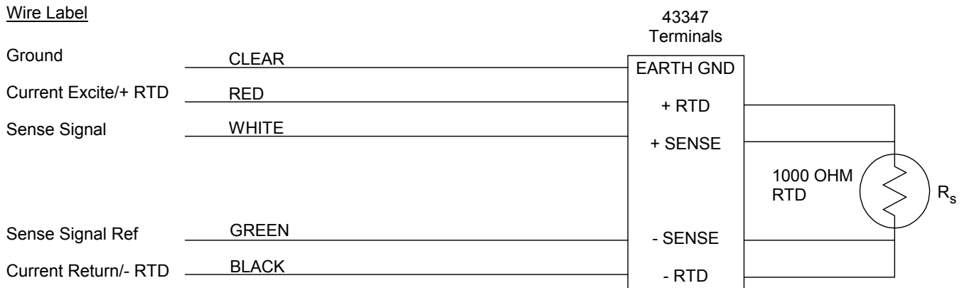
FIGURE 6-1. 43347-IX Temperature Probe Schematic
