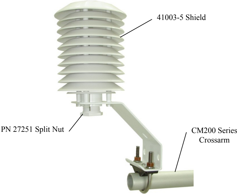
FIGURE 3-4. 41003-5 Radiation Shield Mounted to a CM200 Series Crossarm
