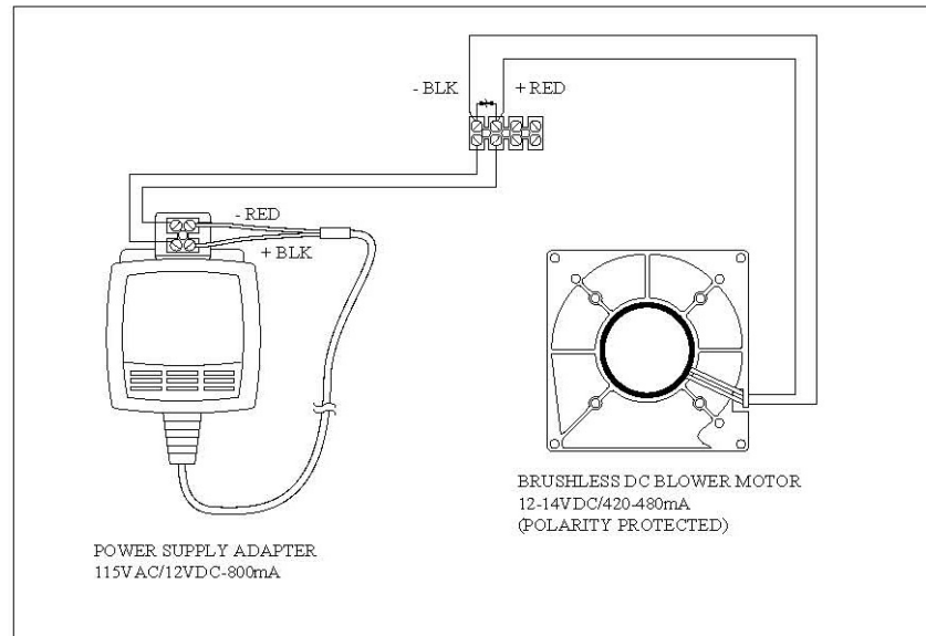
FIGURE C.2-2. 43408 Aspirated Radiation Shield Wiring
