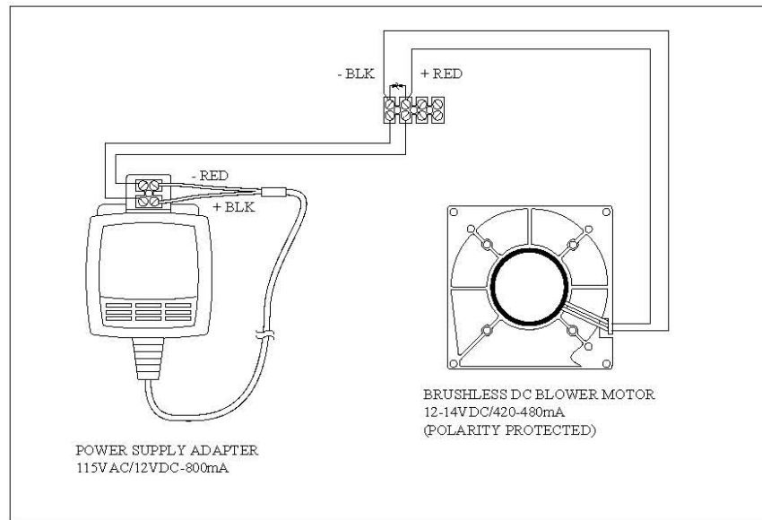
FIGURE 4-2. 43502 Aspirated Radiation Shield Wiring
