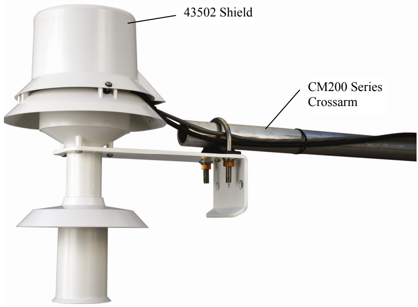
FIGURE 3-2. 43502 Radiation Shield Mounted to a CM200 Series Crossarm
