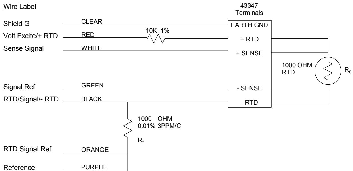
FIGURE 4-1. 43347-VX Temperature Probe Wiring
