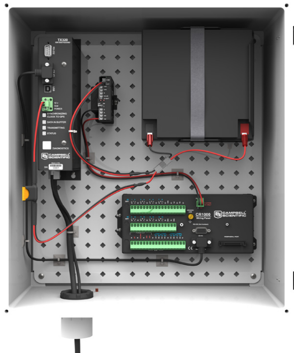
FIGURE 3-3. DCP enclosure
