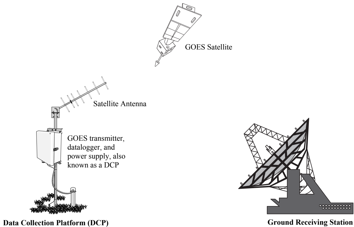
FIGURE 2-1. Major components of the GOES/DCP system (GPS antenna not shown)
