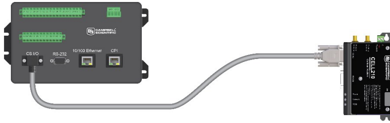
Figure 8-1. CS I/O connection
