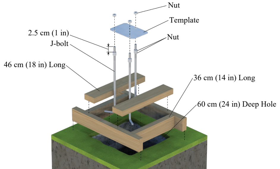
FIGURE 3-2. Base Assembly
