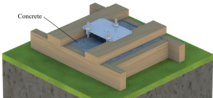
FIGURE 3-3. Base Embedded in Concrete
