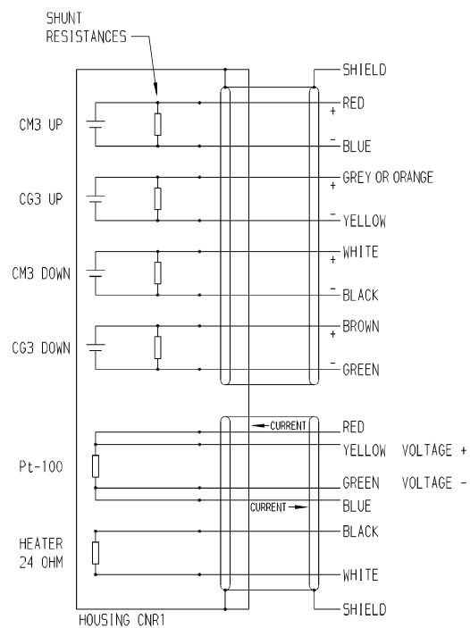
FIGURE 5-1. CNR1 Schematic
