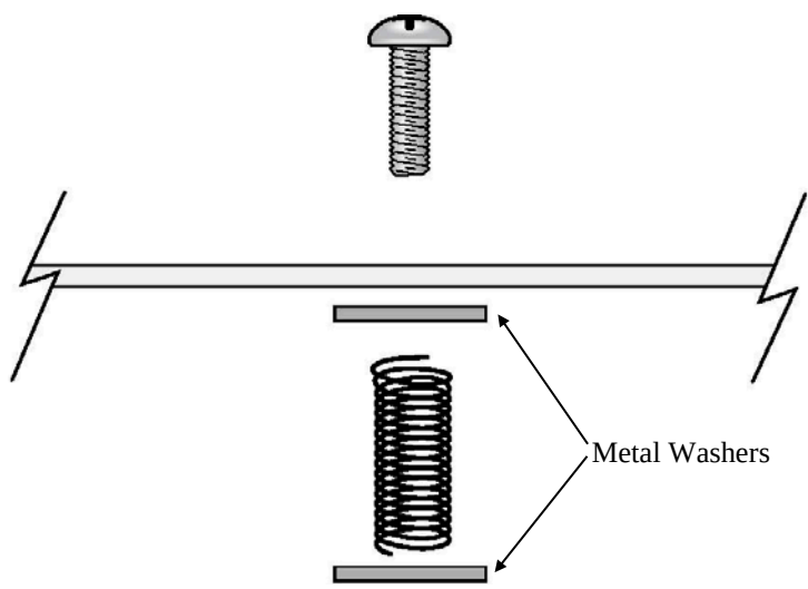
FIGURE 4-6. Installing Leveling Screws
