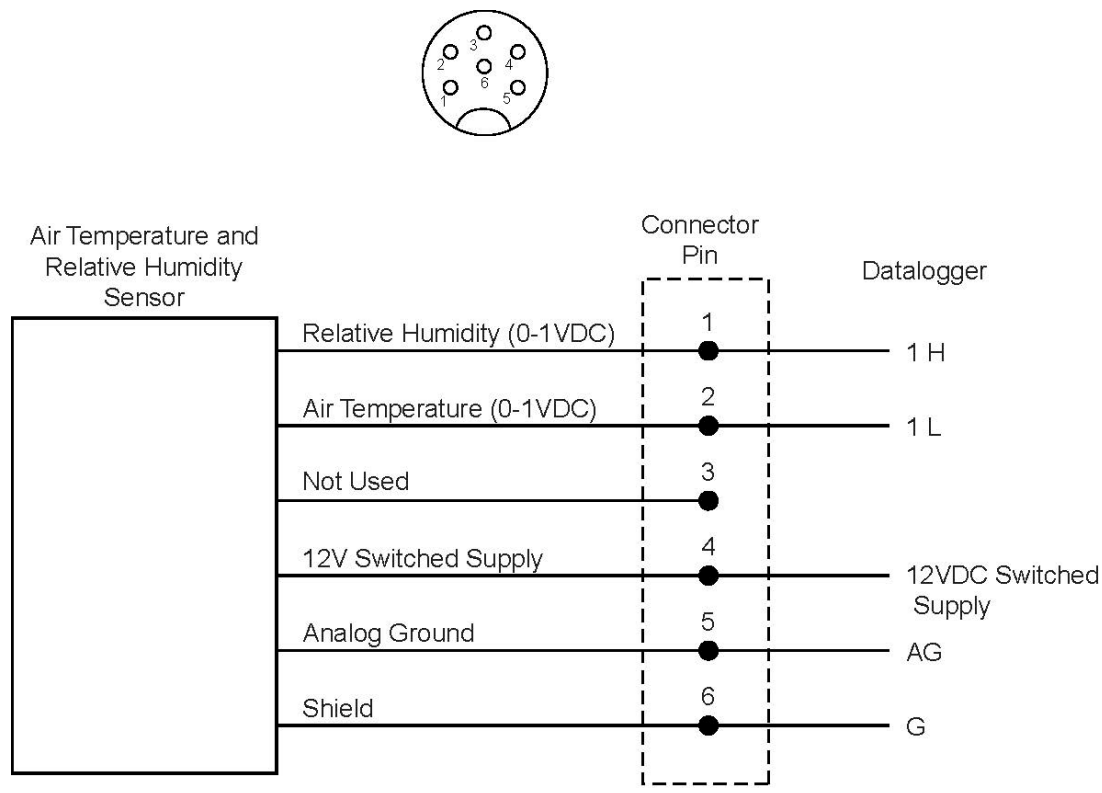
FIGURE 4-7. Schematic of CS500-LC RH and Temperature Probe and Connector #1
