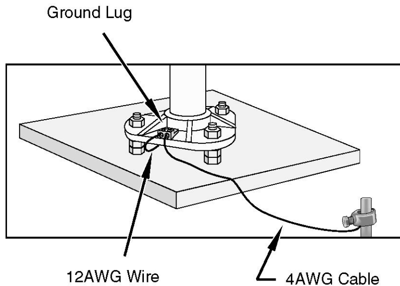
FIGURE 2-3. Raising and Grounding the ET Tower
