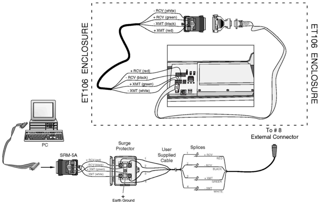
FIGURE 3-12. Short-Haul Modem Wiring Diagram
