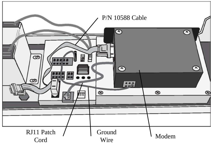
FIGURE 3-8. Phone Modem Mounting and Connections
