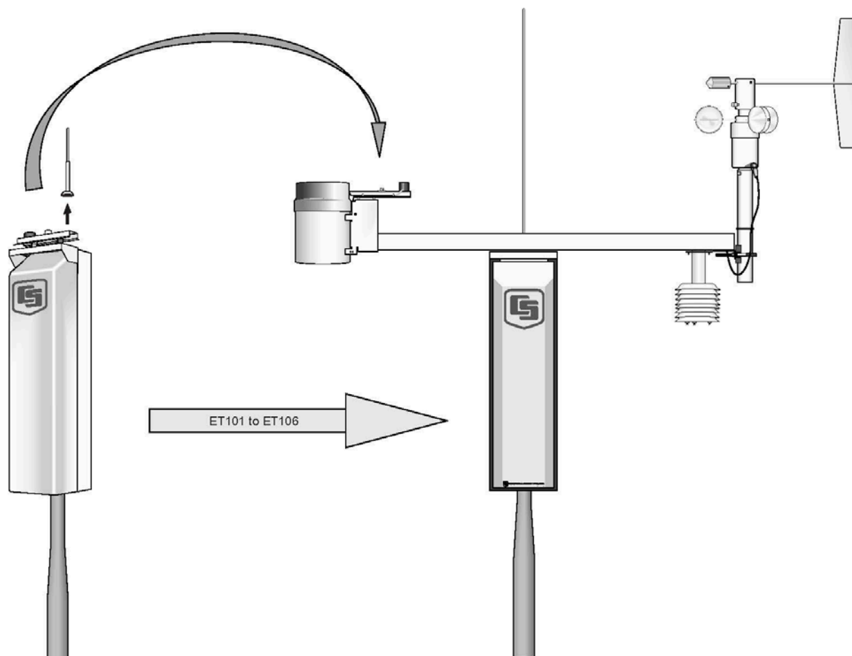
FIGURE 4-4. Upgrading the ET101 to an ET106
