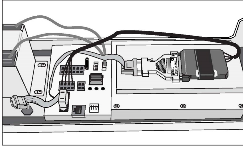
FIGURE 3-11. Short-Haul Modem Mounting and Connection
