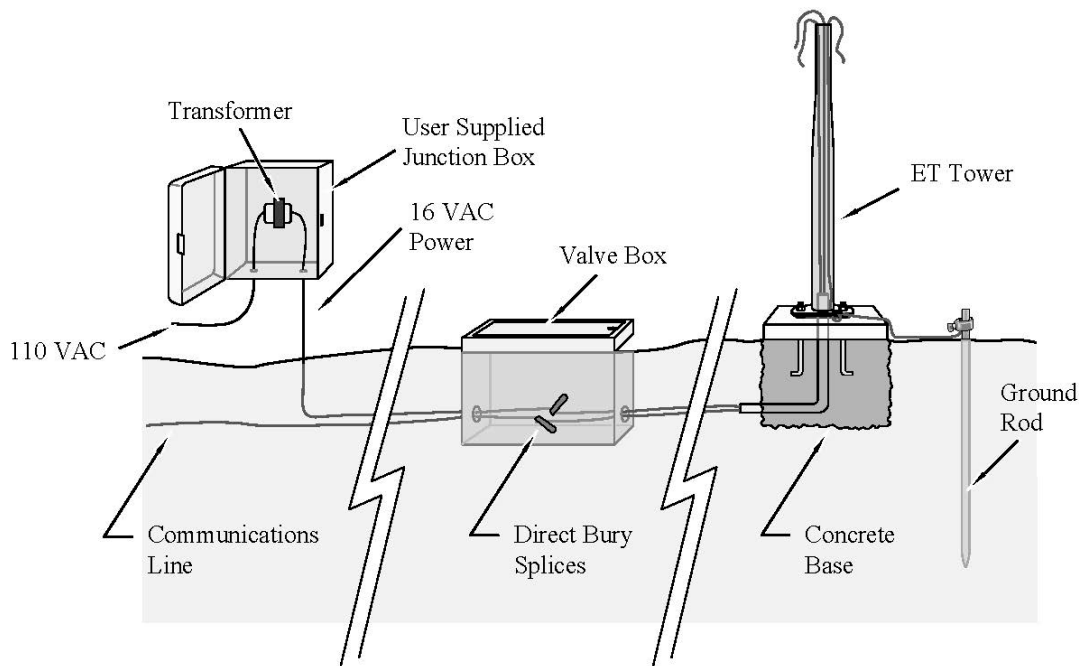
FIGURE 2-1. ET Tower Installation
