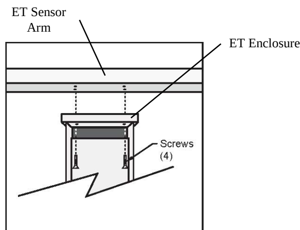
FIGURE 4-1. ET106 Sensor Arm Mounting
