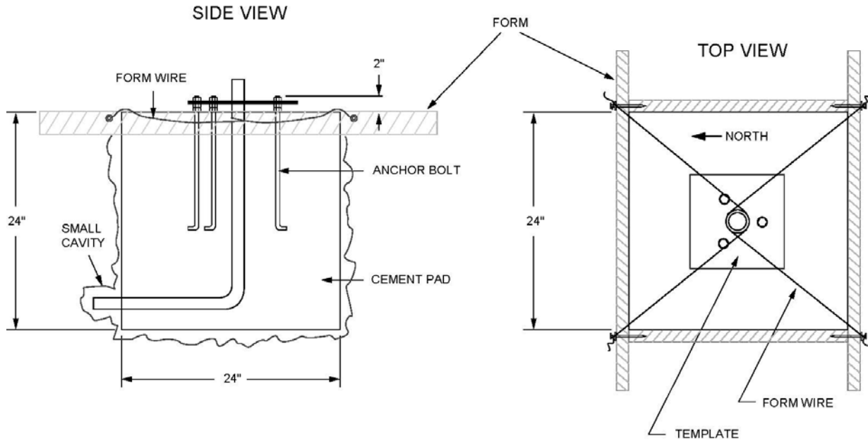
FIGURE 2-2. ET Tower Base Installation
