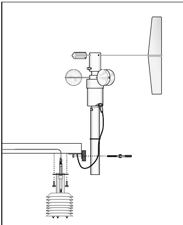
FIGURE 4-2. Wind and RH/Temperature Sensor Installation
