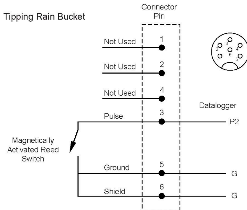
FIGURE 4-10. Schematic of TE525-LC Rain Sensor and Connector #5
