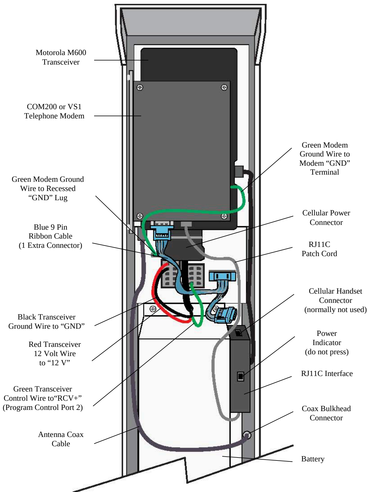
FIGURE 3-9. Cellular Phone Mounting and Connection
