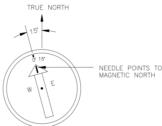
FIGURE 1-4. Declination Angles West of True North Are Added to 0 to Get True North
