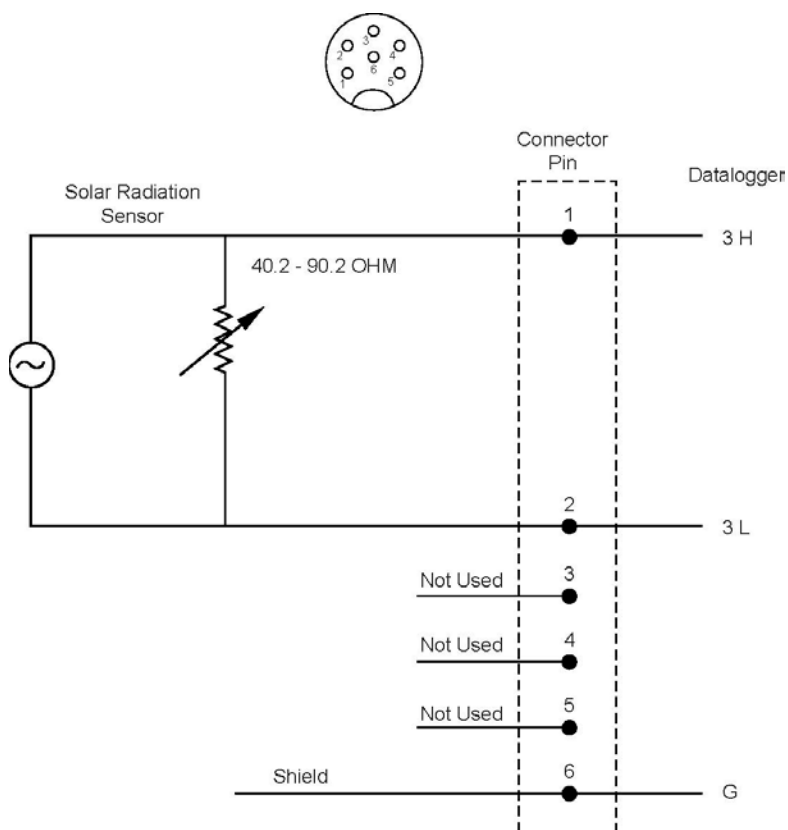
FIGURE 4-9. Schematic of LI200X-LC Solar Radiation Sensor and Connector #3
