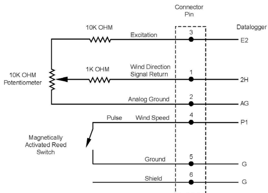
FIGURE 4-8. Schematic of 034A-LC Wind Speed and Direction Probe and Connector #2
