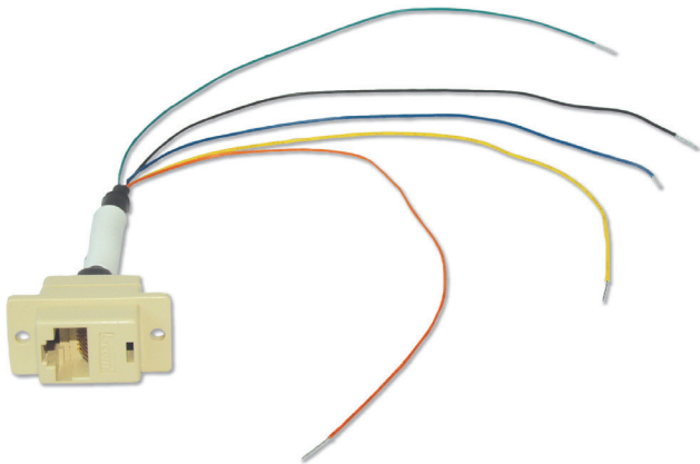
FIGURE 2-1. RJ45 with Flying Leads, Part Number 17217
