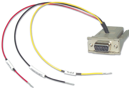
FIGURE 2-3. RJ45 to DB9 Serial Adapter, Part Number 17218
