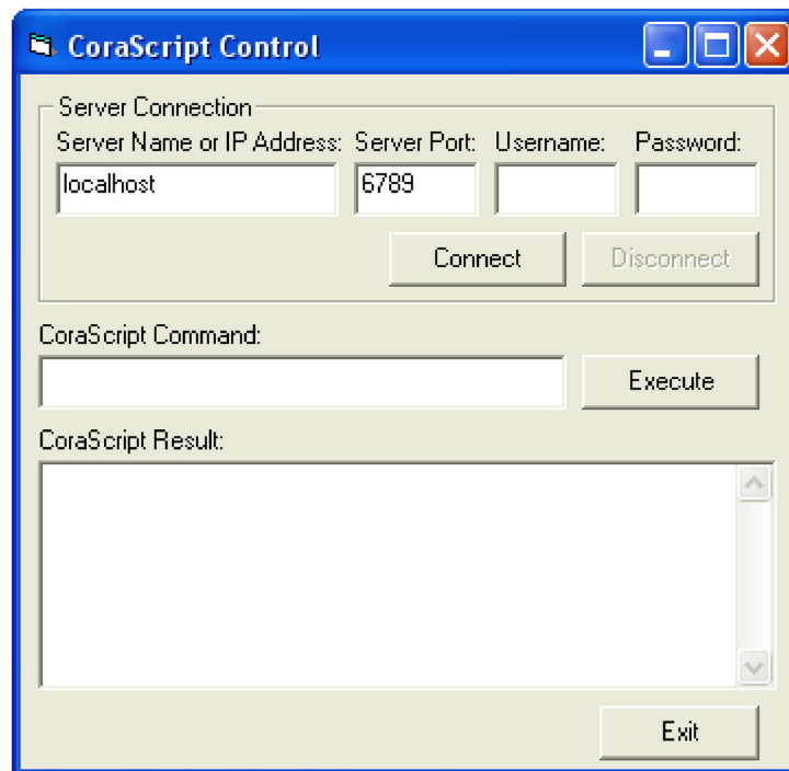
FIGURE 5-1. CsiCoraScript Example
