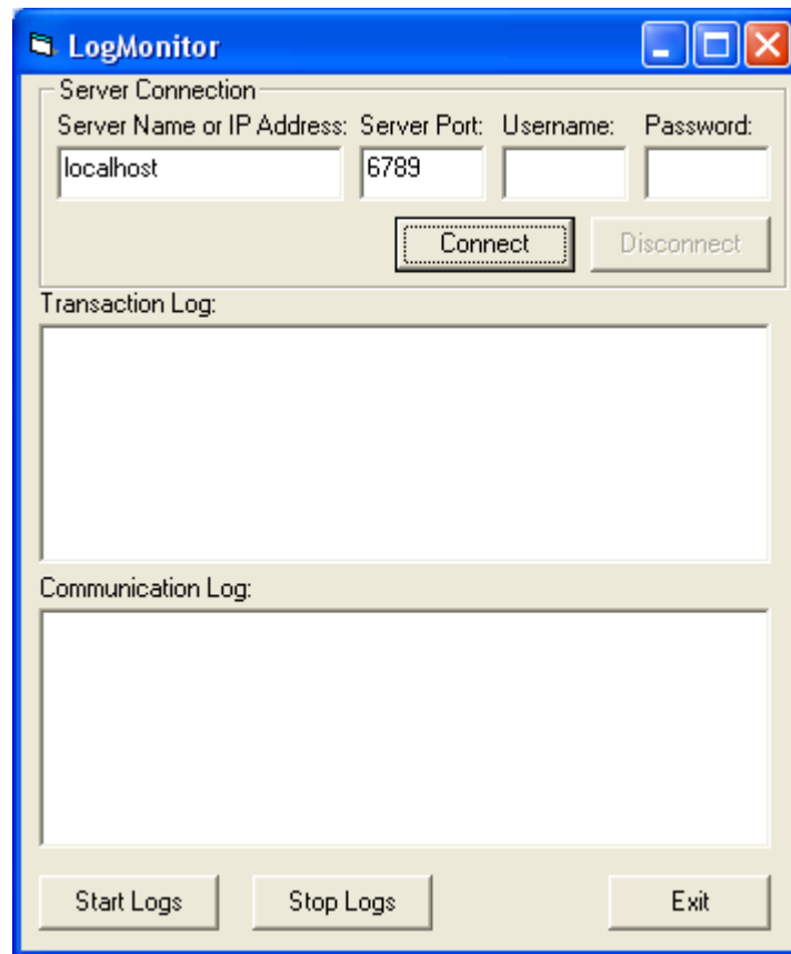
FIGURE 13-1. CsiLogMonitor Example
