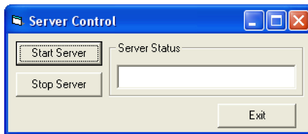
FIGURE 3-1. CsiServer Example
