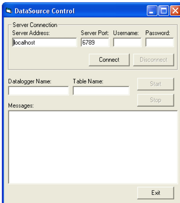
FIGURE 11-1. CsiDataSource Example
