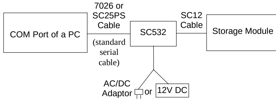
FIGURE 10.2-2. Connecting the Storage Module to a PC using an SC532 Interface
