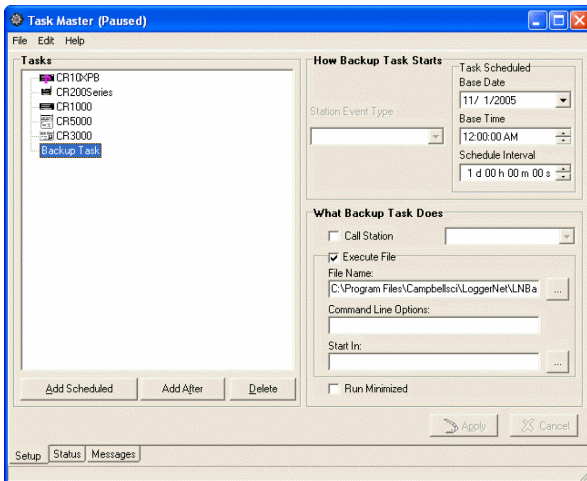
Automatic Backup Configured in Task Master
