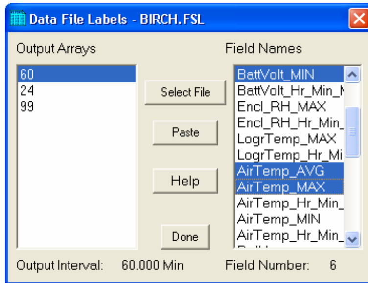
FIGURE 8.2-6. Pasting Labels Into Split
