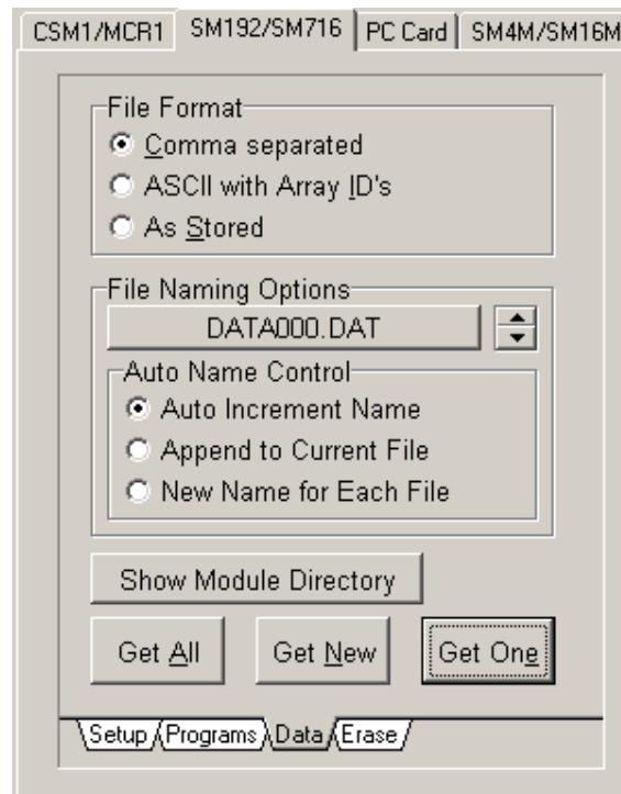
FIGURE 10-5.1. DATA CONTROL Screen
