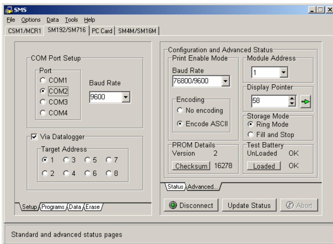
FIGURE 10.2-1. Typical SMS Screen
