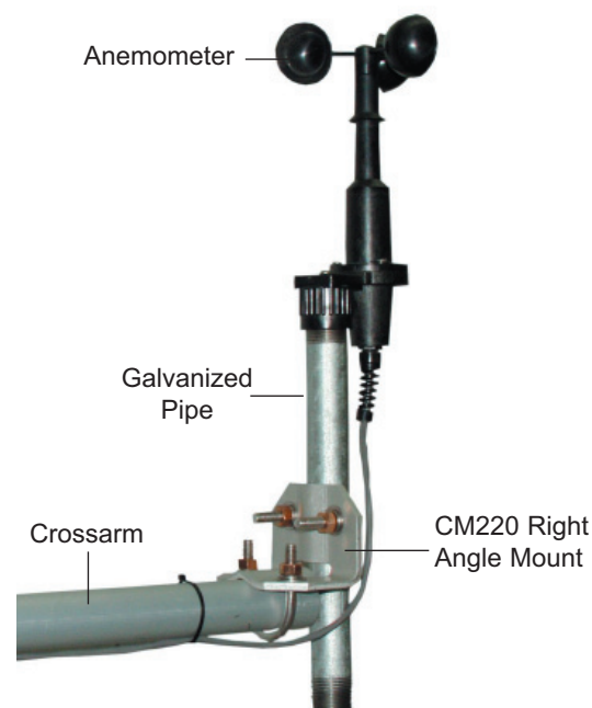
When purchased separately, the Wind Sentry Anemometer is supplied with a galvanized 10" x \frac{3}{4} " -diameter threaded pipe, which mounts to a crossarm via a CM220 Mount or NU-RAIL fitting. Alternately it can mount to an stainless-steel tripod via the CM216.
