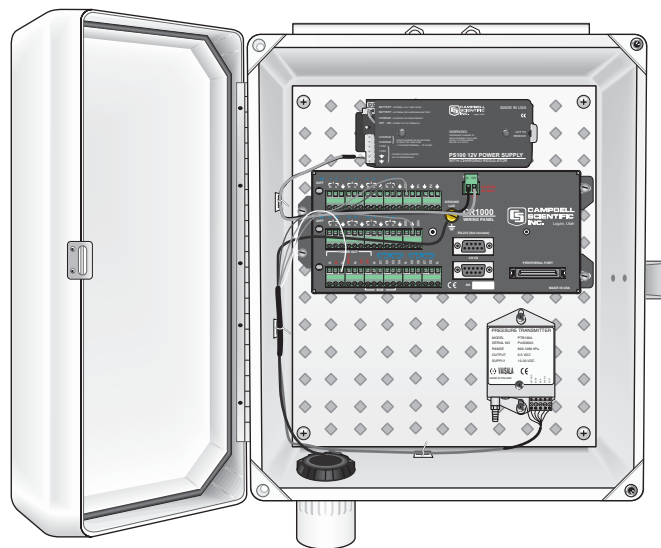
PS100 12 Vdc power supply top, CR1000 datalogger, and CS105 inside ENC12/14 enclosure.
