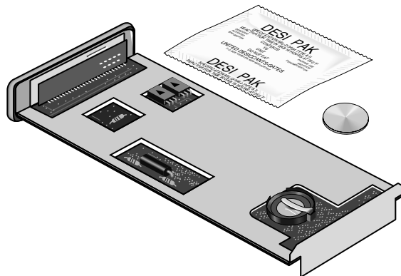
FIGURE 14.11-4. CR10X Lithium Battery Location
