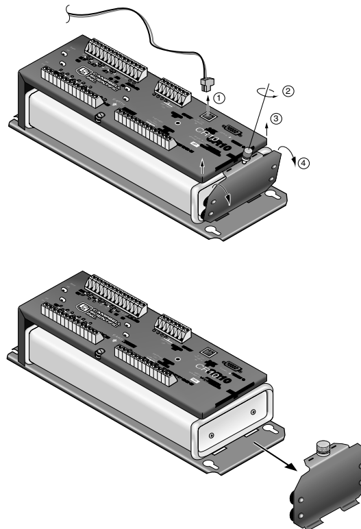
FIGURE 14.11-1. Removing Wiring Panel
