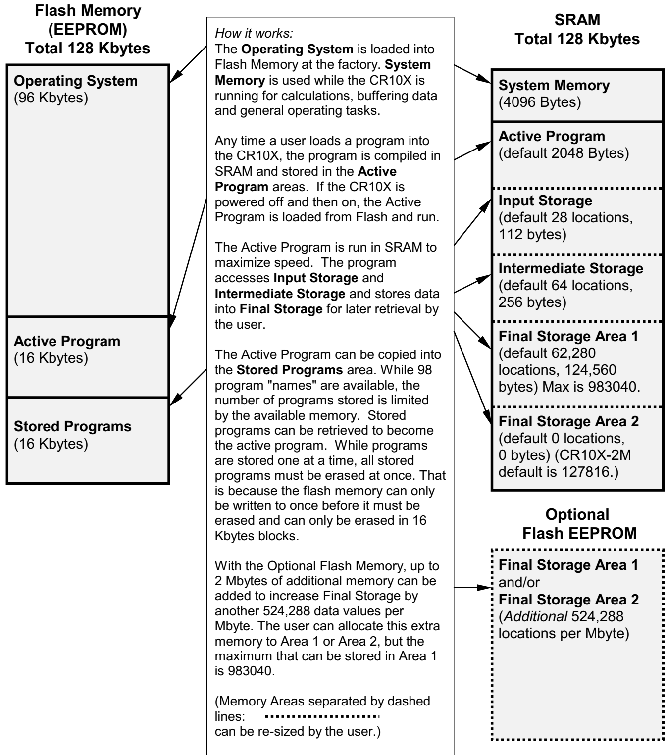
FIGURE 1.5-1. CR10X Memory
