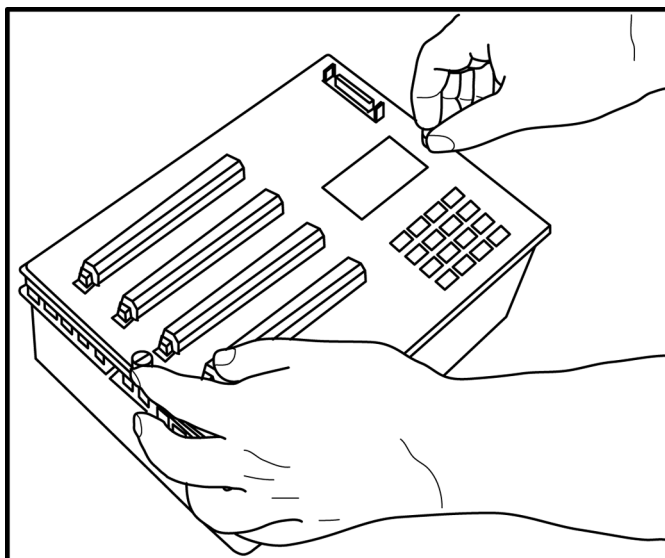
FIGURE 121: Loosen Thumbscrews
