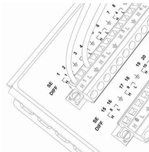
FIGURE 20: Analog Sensor Wired to Differential Channel #1
