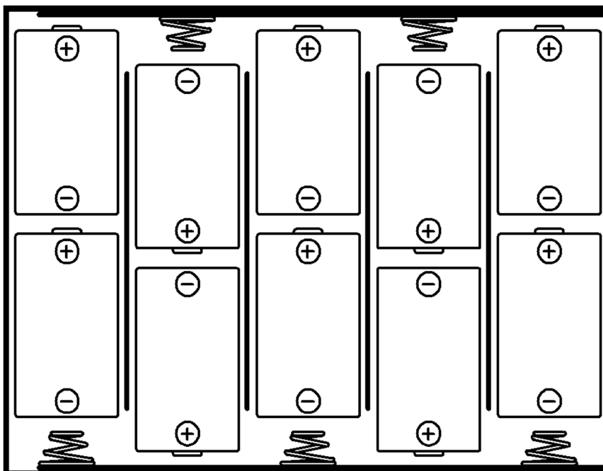
FIGURE 30: Alkaline Battery Orientation
