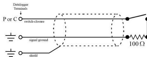
FIGURE 102: Current-Limiting Resistor in a Rain Gage Circuit
