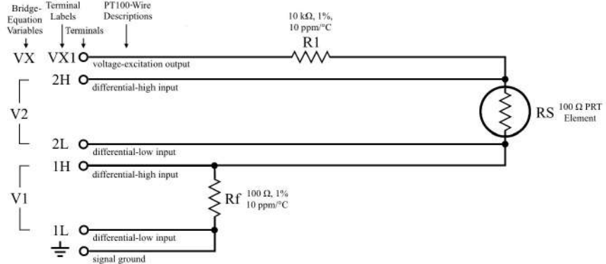
FIGURE 67: PT100 BrHalf4W() Four-Wire Half-Bridge Schematic
