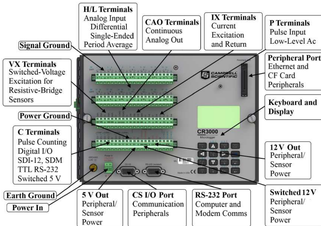
FIGURE 1: Wiring Panel
