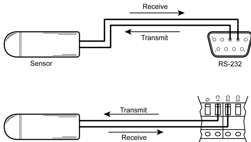
FIGURE 26: Use of RS-232 and Digital I/O when Reading RS-232 Devices
