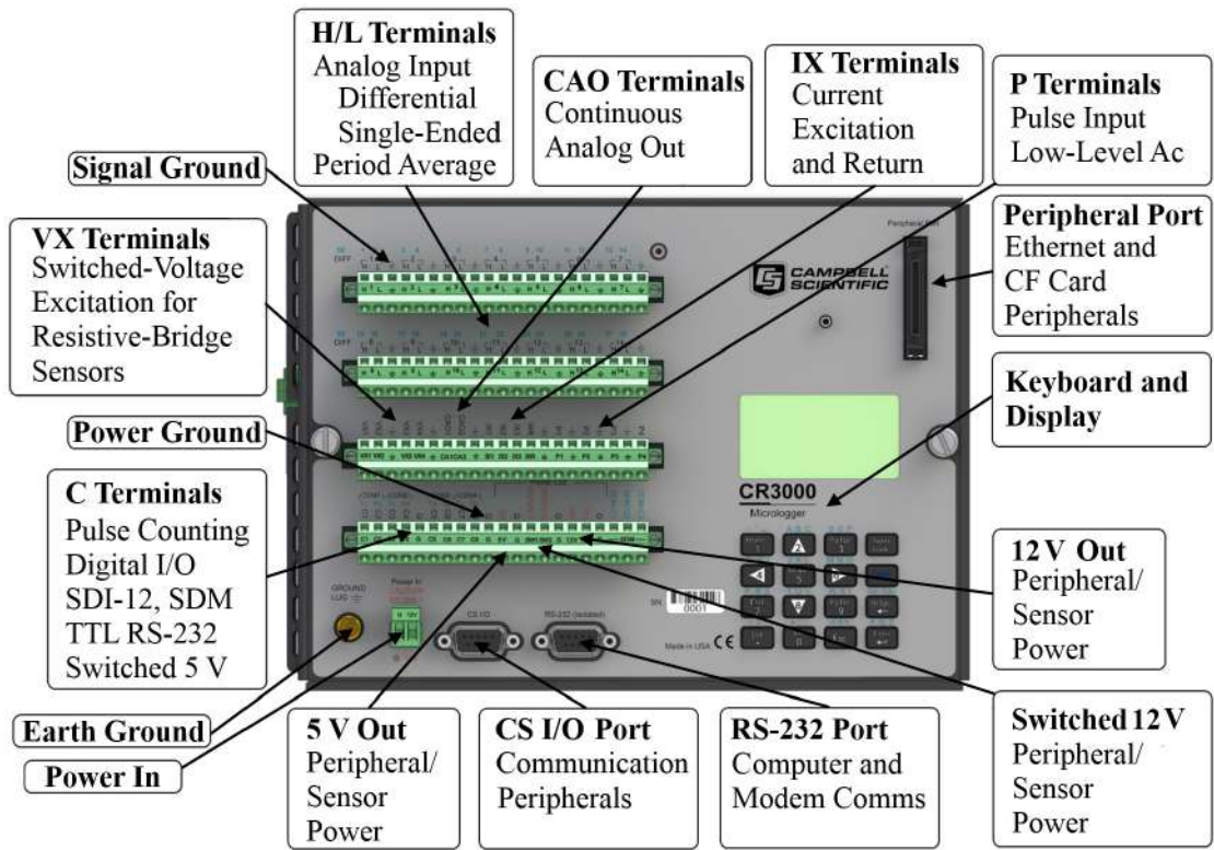
FIGURE 17: Wiring Panel
