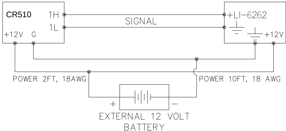
FIGURE 7.2-1. Typical Connection for Active Sensor with External Battery
