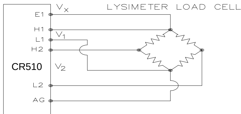
FIGURE 7.10-2. 6 Wire Full Bridge Connection for Load Cell
