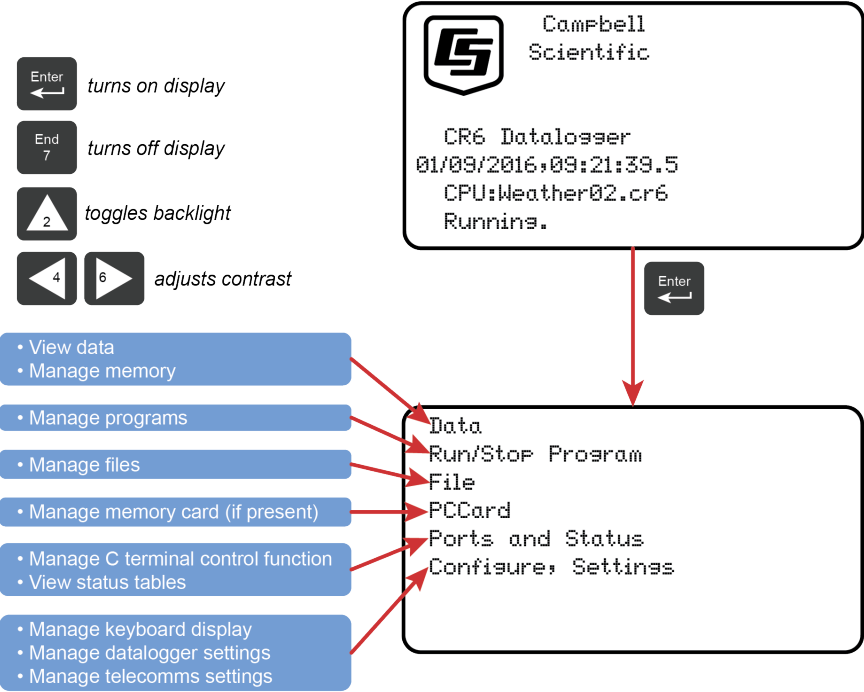
FIGURE 99: CR1000KD: Navigation
