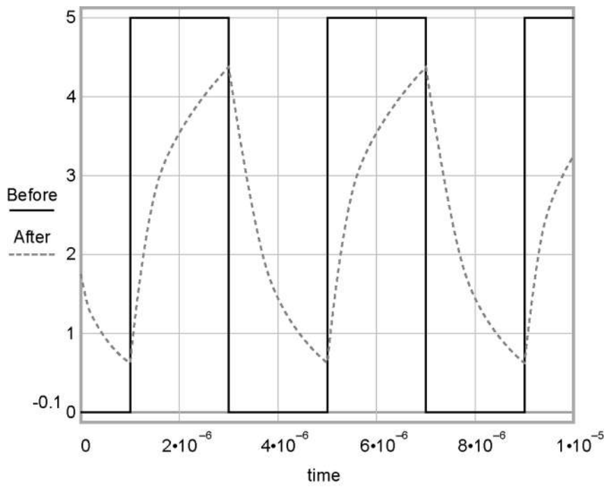
FIGURE 88: Amplitude reduction of pulse count waveform (before and after 1 \mu s \mu s time-constant filter)
