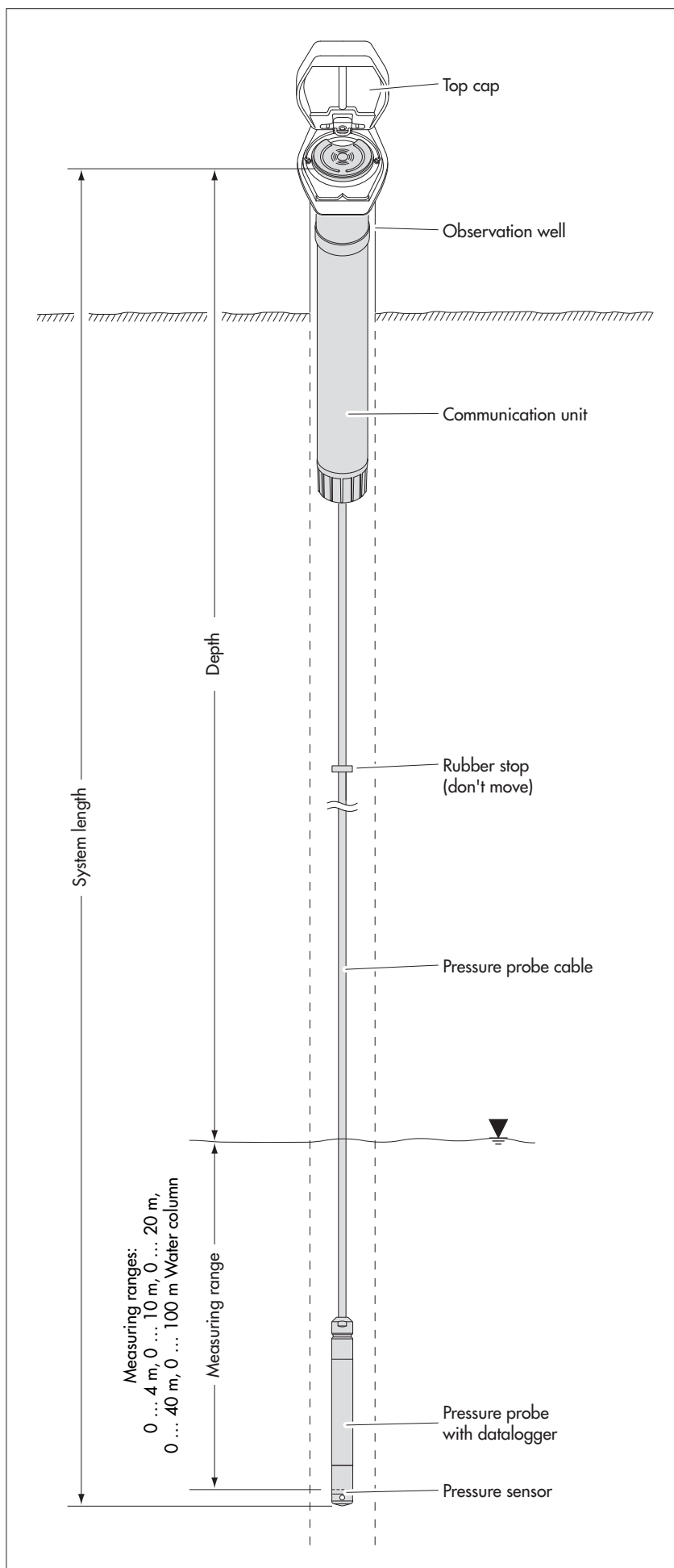
Fig. 1: Setup of a groundwater measurement station using the OTT ecoLog 500 (3G).
