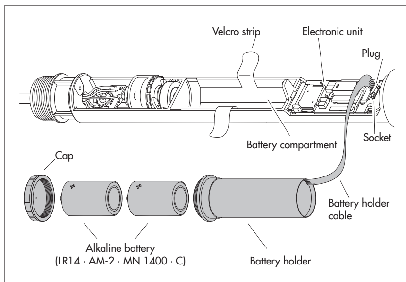
Fig. 4: Inserting alkaline batteries into the battery holder.
