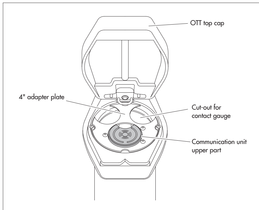
Fig. 12: Installing the OTT ecoLog 800 (3G) into a 3", 4" or 6" observation well. Example: 4" observation well.
