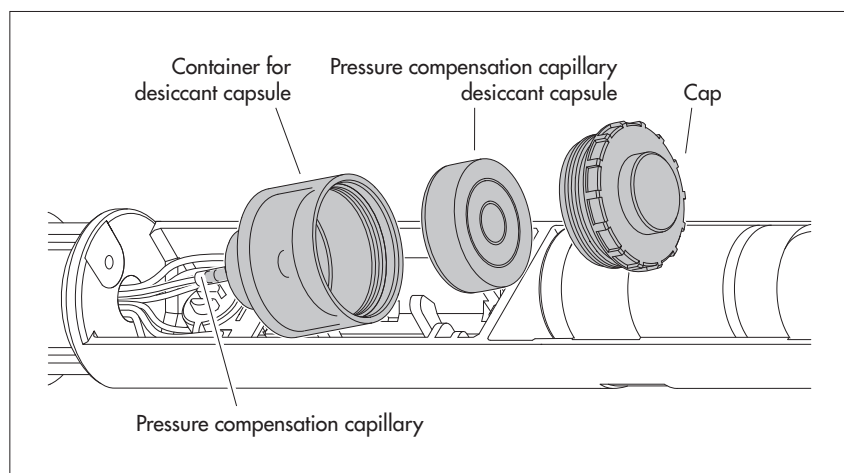
Fig. 28: Replacing the pressure probe desiccant capsule.
