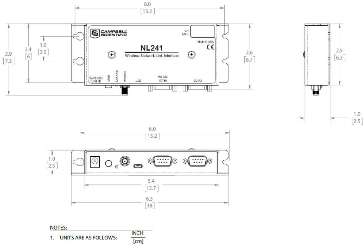
FIGURE 5-1. NL241 dimensions
