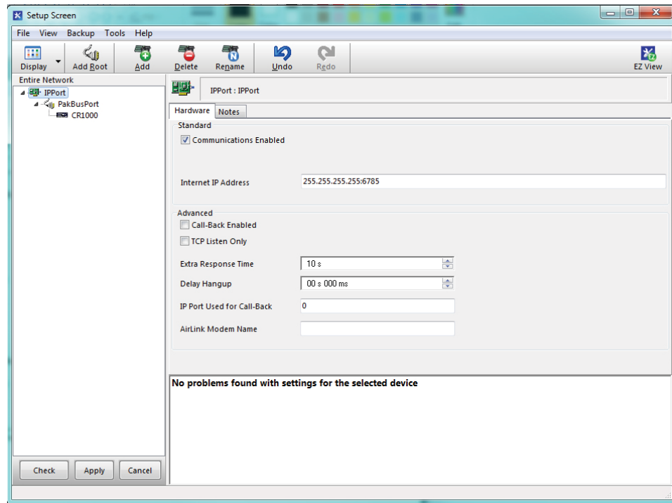
Figure 6—2 Example of Static IP Setup
