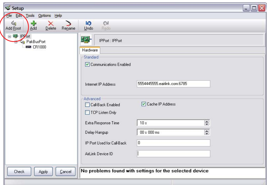
Figure 6—1 Example of Dynamic IP Setup
