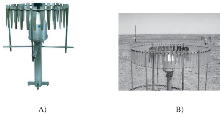
FIGURE 6—2. A) T-200B with 1.2 m diameter Alter wind screen, mounted to pedestal. B) T-200B with 2.4 m Alter wind screen.
