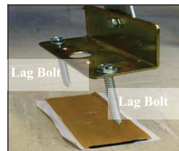
Figure 11: The TP1 Tripod Kit includes the lag bolts used to secure the TP1 to a roof. Two lag bolts are used for each tripod foot. The bolts must pierce the sealing pads.
