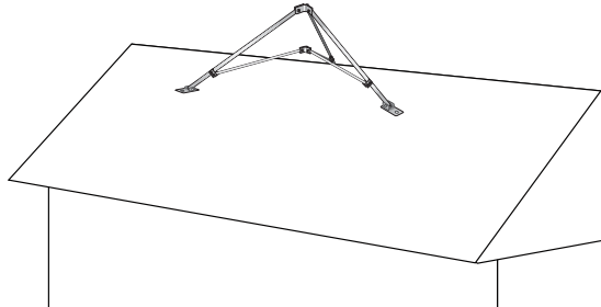
Figure 10: Proper placement of the tripod on a peaked roof. When properly placed, all foot pads rest flat on the roof.
