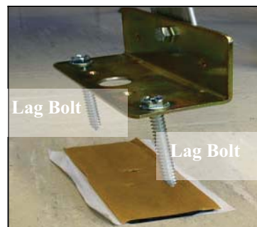
Figure 8: The TP1 Tripod Kit includes the lag bolts used to secure the TP1 to a roof. Two lag bolts are used for each tripod foot. The bolts must pierce the sealing pads.
