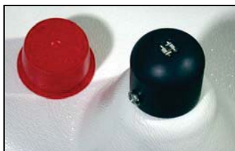
Figure 16: The red cap (left) protects the solar radiation sensor (right) while the WeatherHawk is being shipped and installed. Accurate measurements require the cap to be removed.
