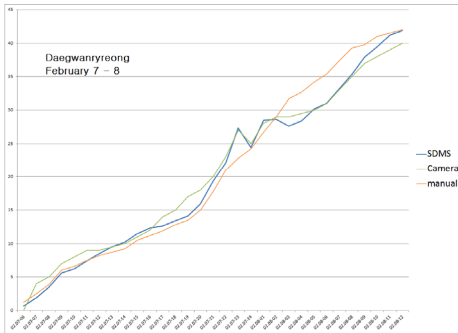
Figure 11 Measurements at site 3 on 2/7/2014 and 2/8/2014 unit: mm
