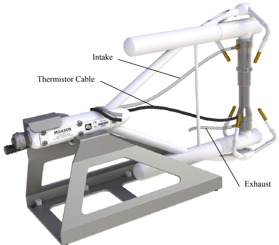
FIGURE 9-4. The zero-and-span shroud mounted on the zero-and-span stand. The top tube is the gas intake, the black cable is the temperature thermistor, and the short bottom tube is the gas exhaust.
