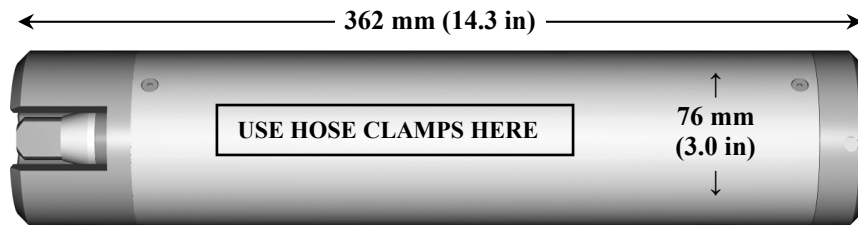
FIGURE 5-1. Dimensions
