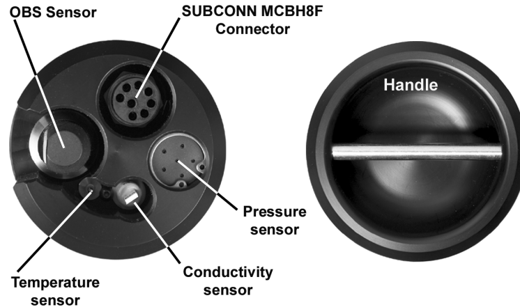
FIGURE 6-1. Components
