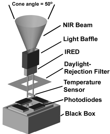
FIGURE 4-1. Anatomy of an OBS sensor
