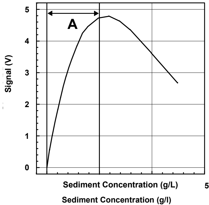
FIGURE 10-3. Response at high sediment concentrations
