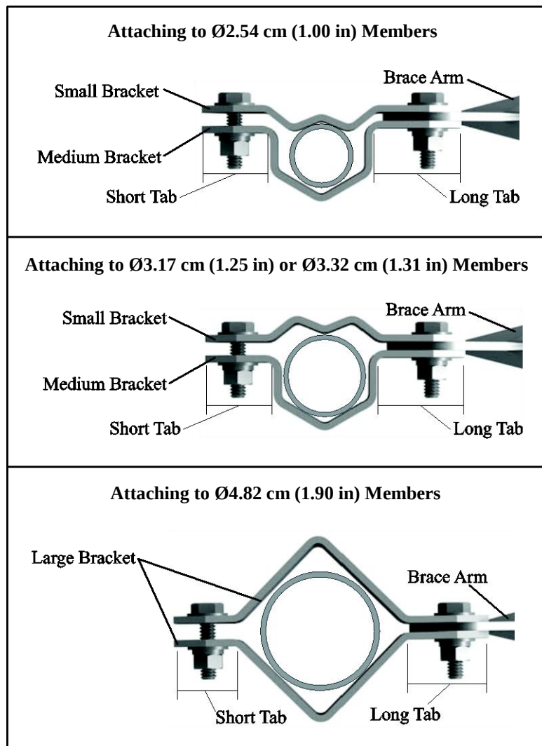
Figure 6-18. Bracket selection
