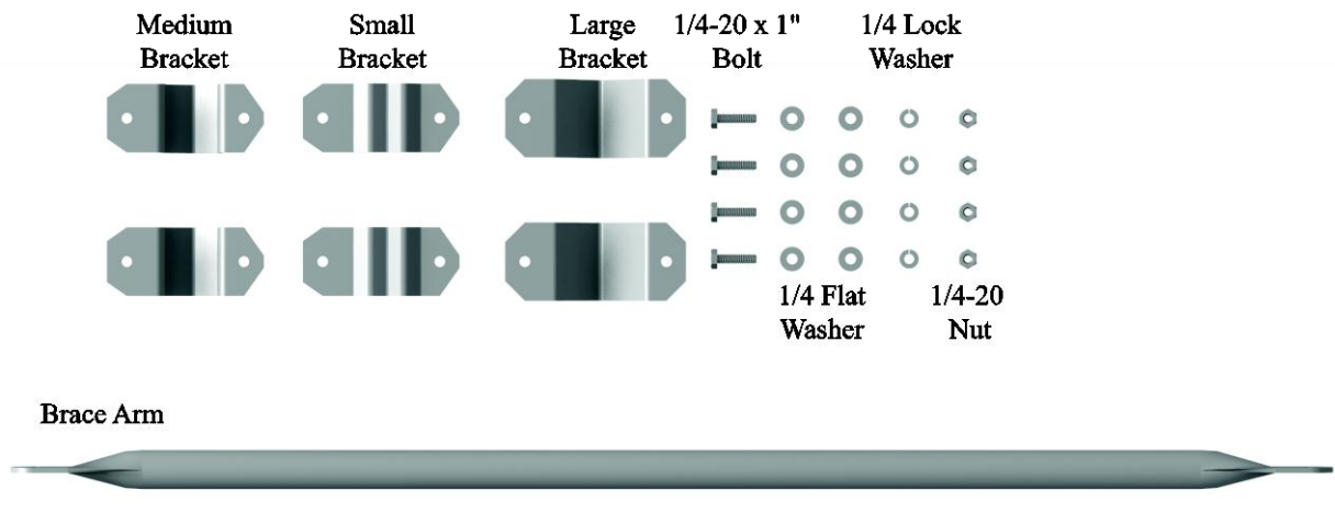
Figure 6-17. CMB200 components
