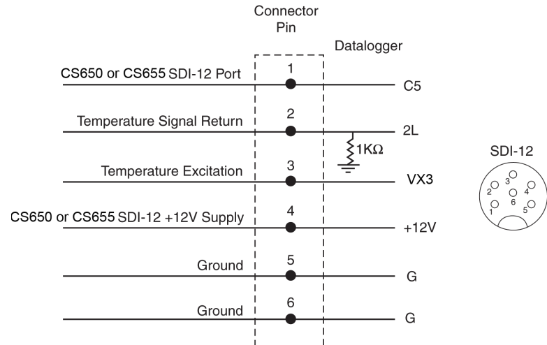
FIGURE 8-7. Schematic of CS650-LC or CS655-LC
