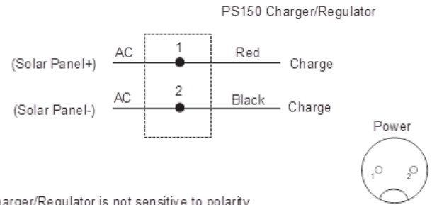
FIGURE 8-8. Schematic of solar panel and connector Power
