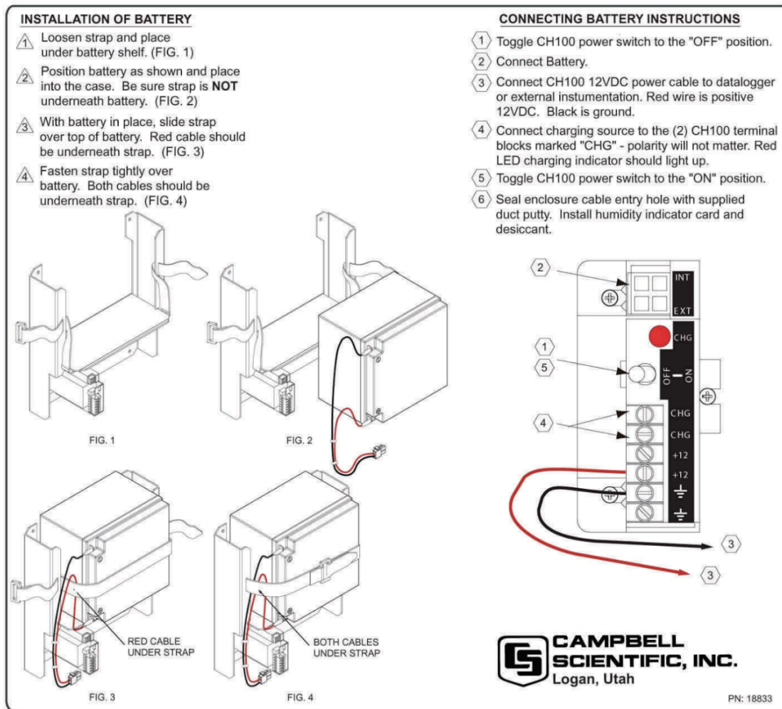
FIGURE C-10. Procedure for installing and connecting battery
