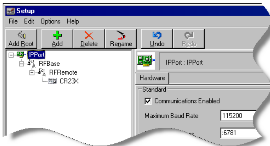
Figure 5. LoggerNet Setup for NL100/105 to RF to Datalogger Connection
