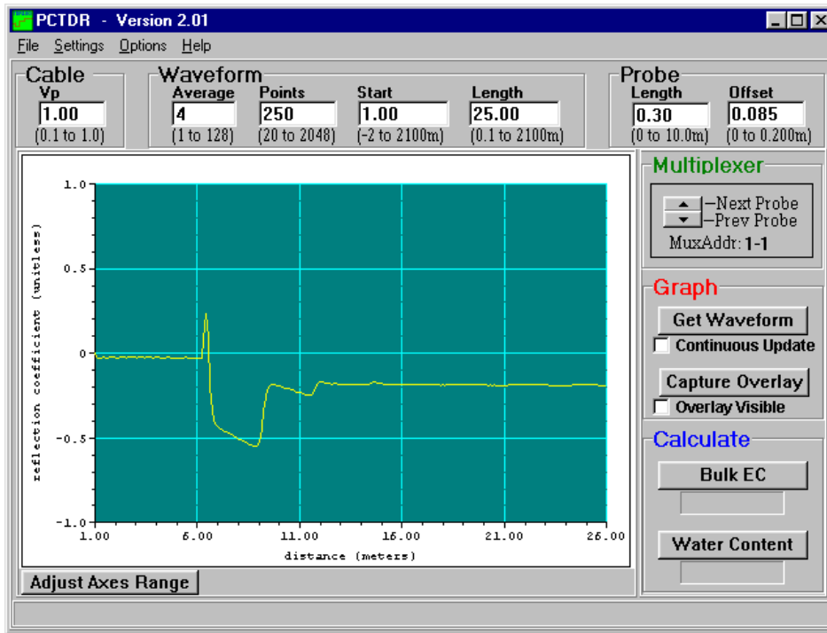
Figure 4-1. Waveform of a CS610 in water
