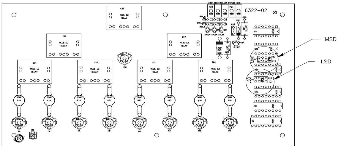
Figure A-2. Location of address jumpers on SDM50
