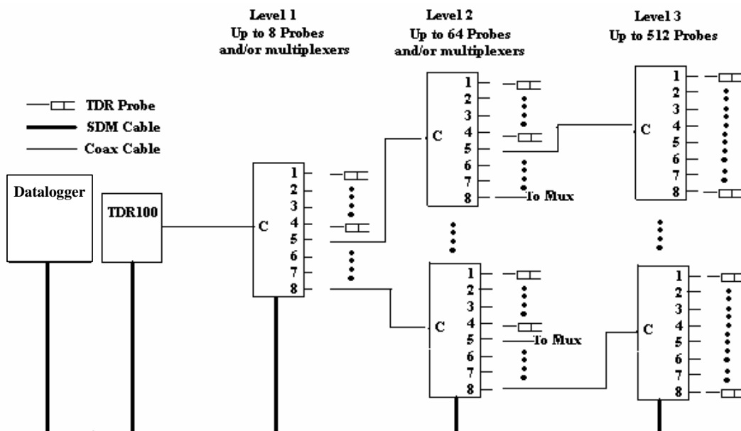
Figure 7-2. TDR system components
