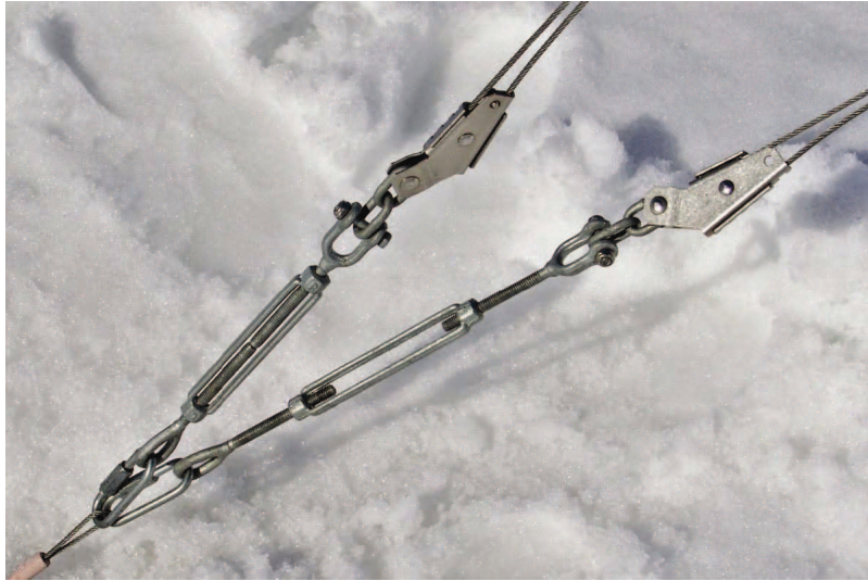
FIGURE 2.4-7. Top and Bottom Guy Cables Fastened to an Anchor
