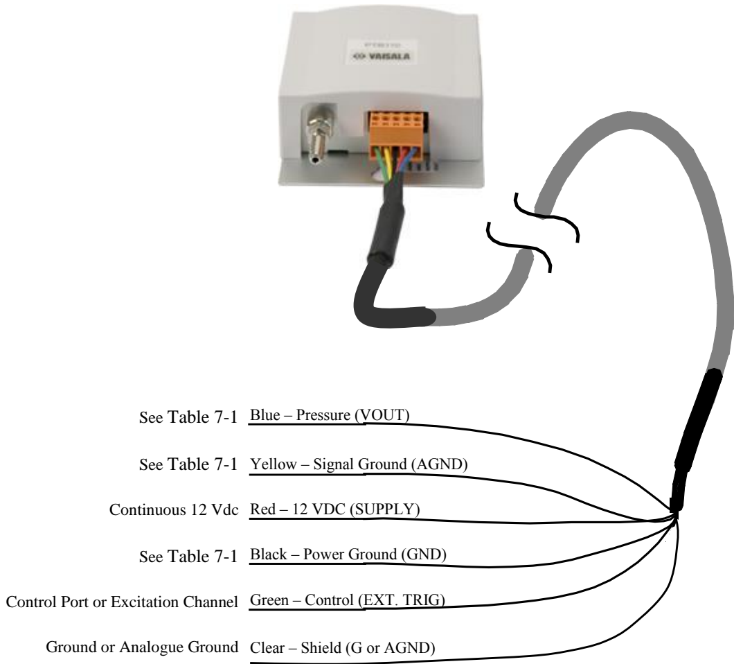
Figure 7-3. CS106 wiring diagram
