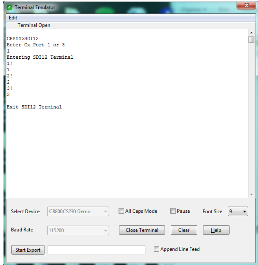
FIGURE 7-1. Screen capture of SDI-12 transparent mode on CRBasic CR800 datalogger using control port 1 and prompting for SDI-12 addresses
