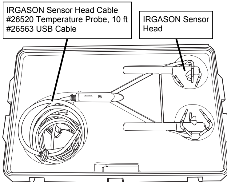
FIGURE 1. Foam Cutout and Components in Upper Level of Packaging
