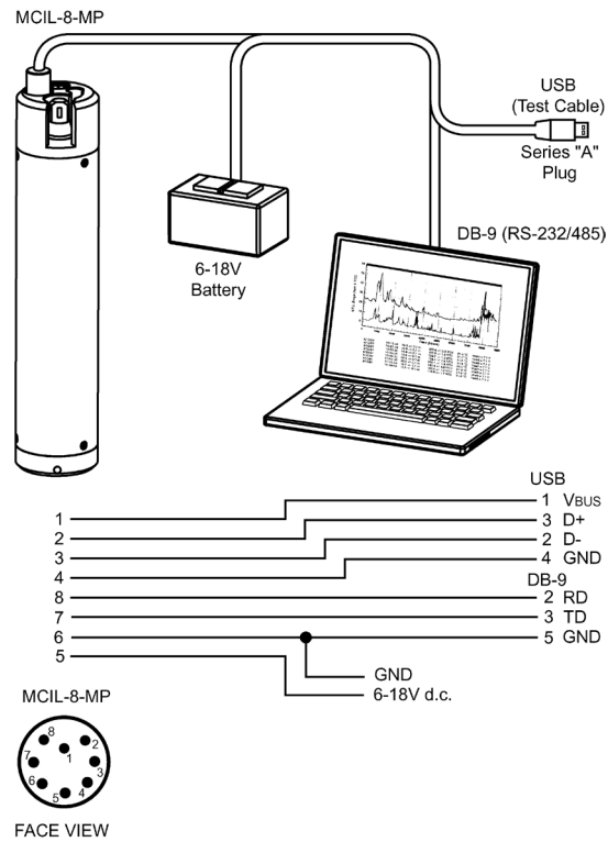
FIGURE 6-3. Connections and wiring of field cable
