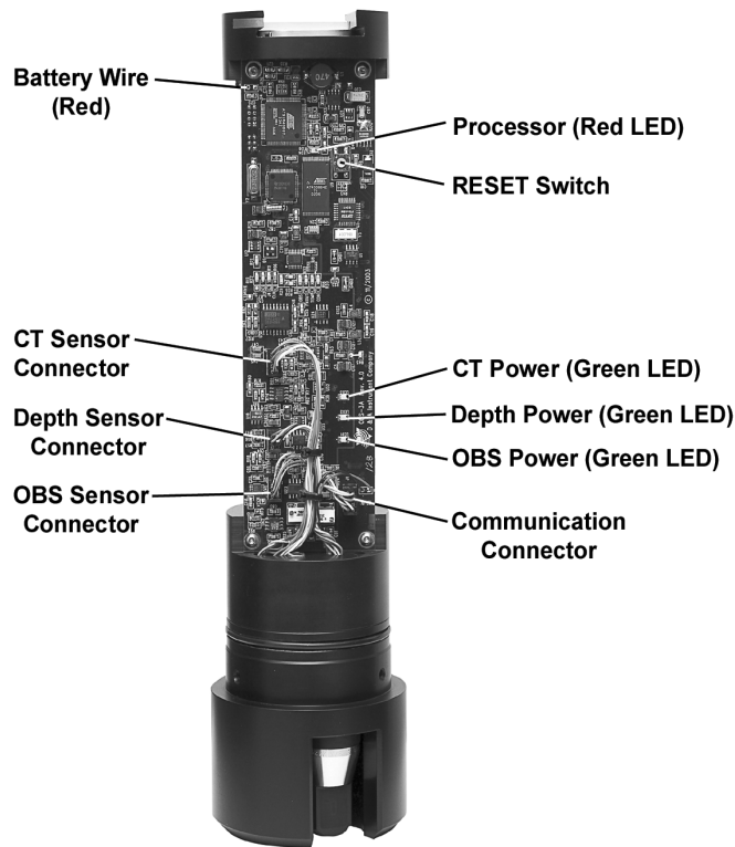
FIGURE 8-1. Component locations
