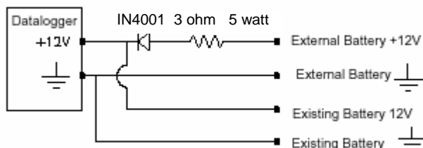
Figure 6. Connecting to External Power Supply
