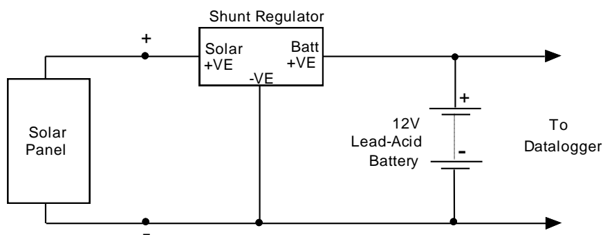
Figure 5. Connection of Shunt Regulator for SP10R Panels
