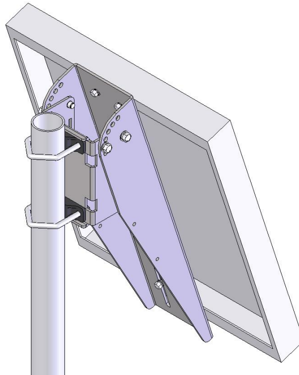
Figure 3b. Solar panel mounted on pole using the multi-mount bracket
