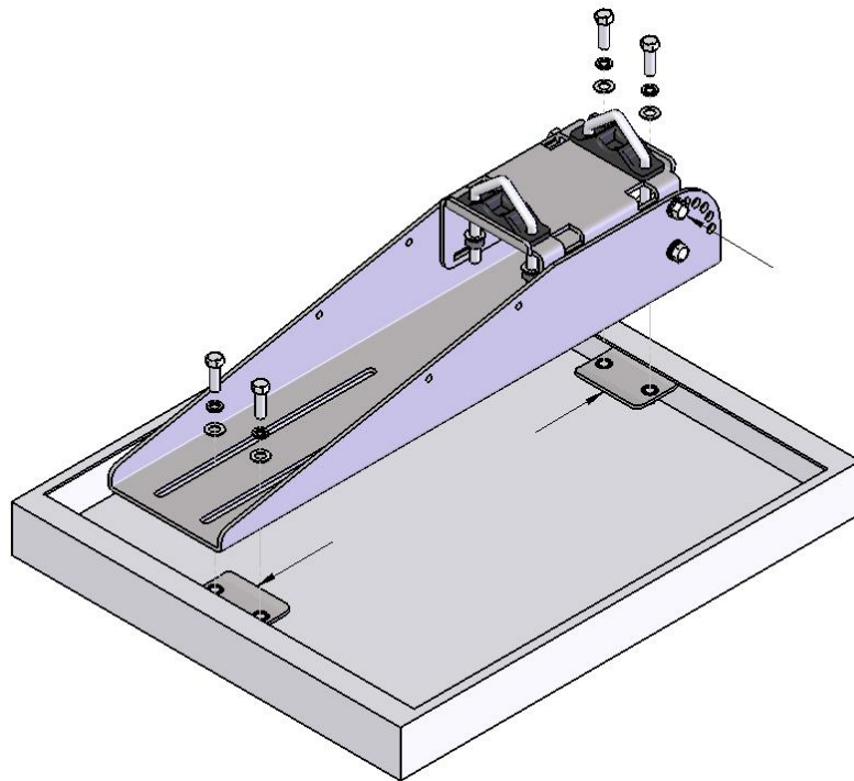
Figure 3a. Assembly drawing for fitting the multi-mount bracket to a larger panel
