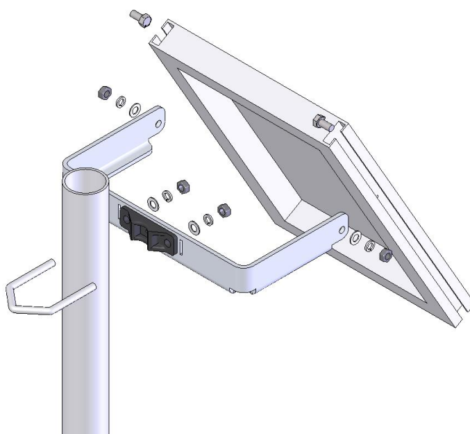
Figure 2. Assembly details of bracket for the SP5 and SP10
