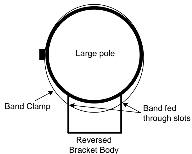
Figure 4. How to attach the multi-fit bracket to larger poles using a band clamp
