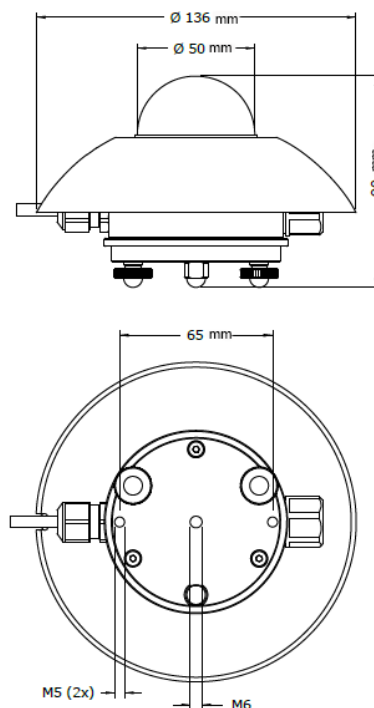
FIGURE 5-1. SR11 dimensions
