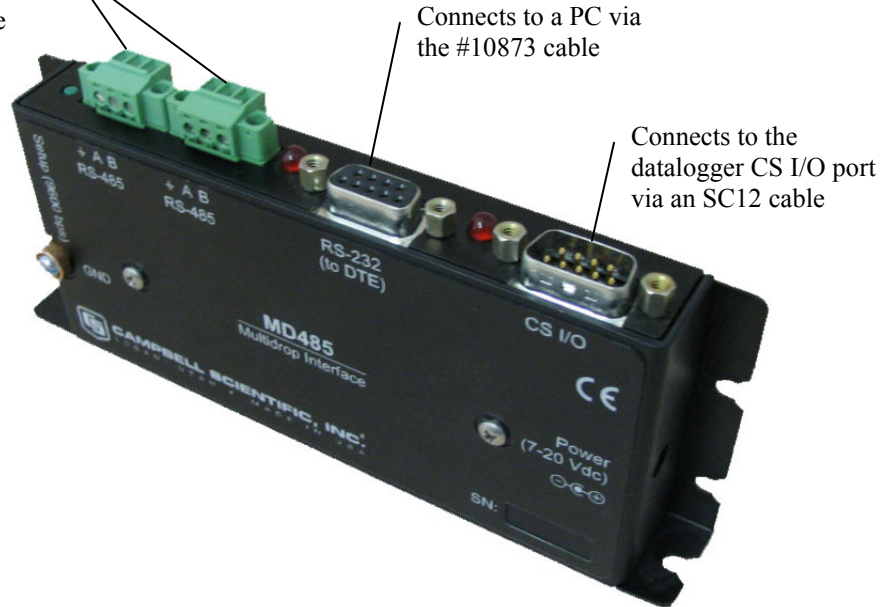
FIGURE 3.3-5. You can configure any two types of interface ports (RS-485, RS-232, and CS I/O) to be used at a time
