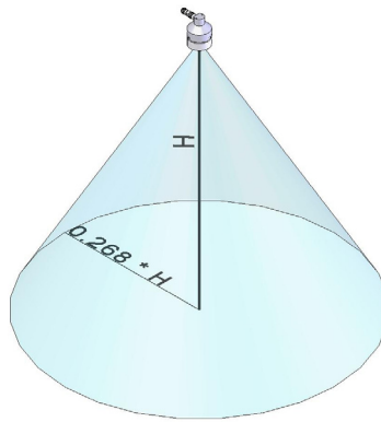
FIGURE 4.12-1. Beam angle clearance
