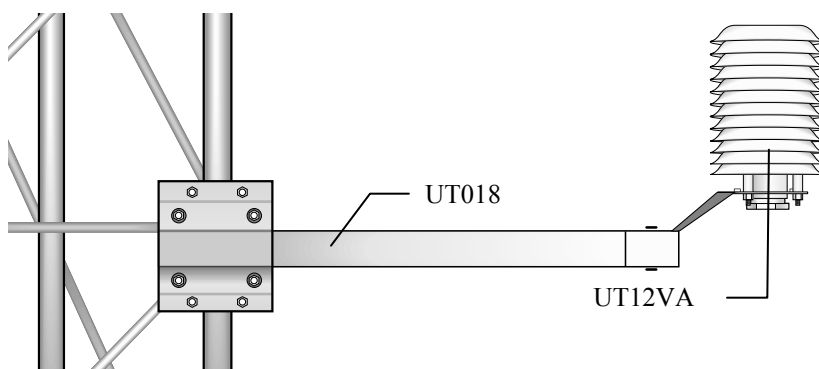
FIGURE 2.2-3. UT12VA Gill Radiation Shield and UT018 Crossarm
