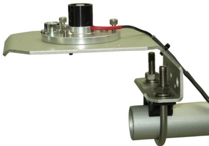
FIGURE 2.2-5. CM225 Solar Radiation Mount with a LI2003S Leveling Base and LI200X Solar Radiation Sensor
