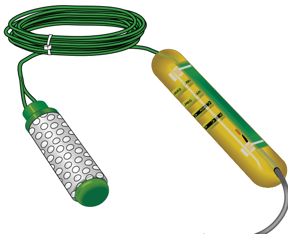
FIGURE 4.15-1. 257 Soil Moisture Sensor
