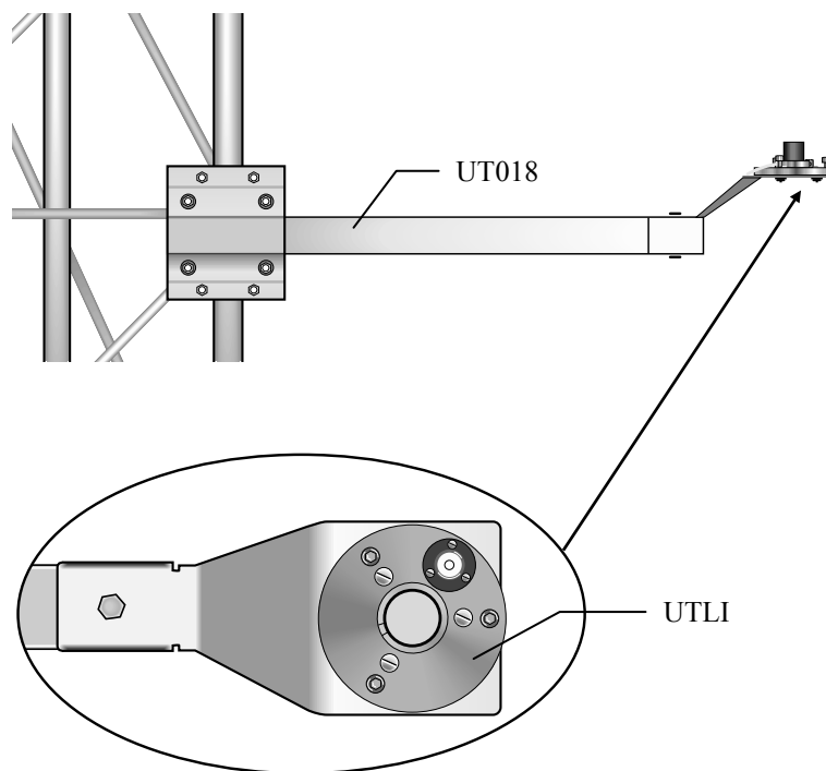
FIGURE 2.2-4. UTLI Leveling Fixture/Crossarm Mount and UT018
