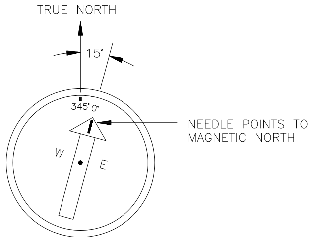
FIGURE 4.17-2. Declination angles east of True North are subtracted from 360 to get True North
