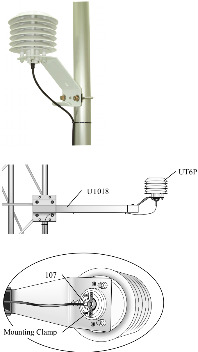
FIGURE 4.5-1. 107 Temperature Probe
