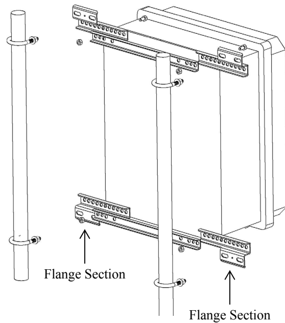
FIGURE 3.1-2. This exploded view shows the components of a “-TM” bracket option
