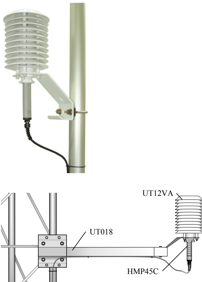
FIGURE 4.8-1. HMP45C Vaisala Temperature and RH Probe
