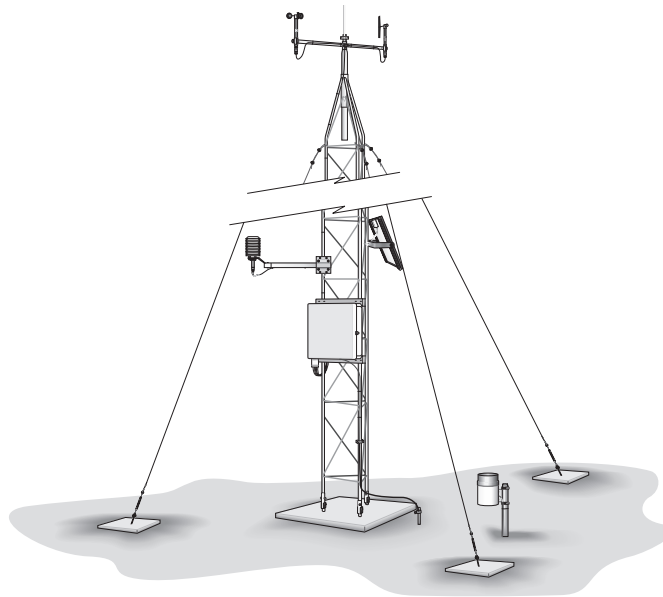
FIGURE 2.1-1. UT30 Tower-Based Weather Station
