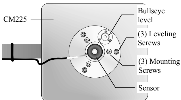
FIGURE 4.4-1. LI200X/LI200S/LI190SB and LI2003S Leveling Fixture
