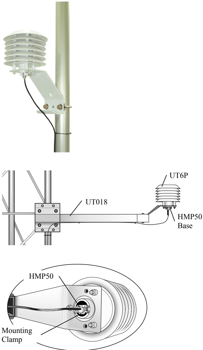
FIGURE 4.7-1. HMP50 Temperature and RH Probe
