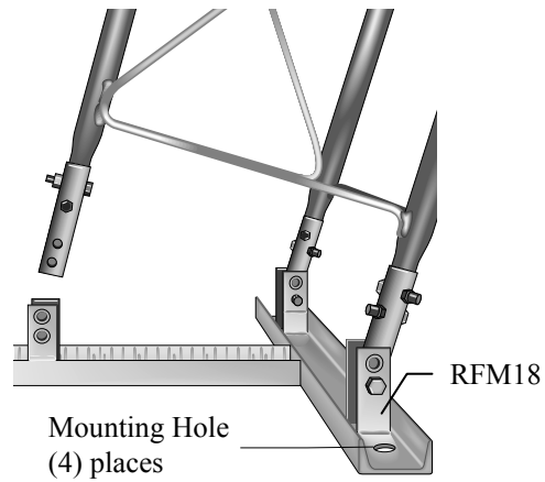
FIGURE 2.1-5. RFM18 flat roof mounting base
