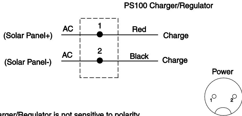
FIGURE 4-10. Schematic of Solar Panel and Connector Power
