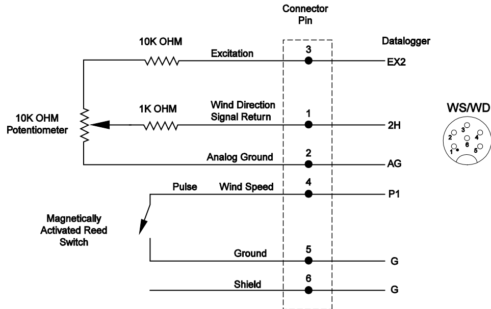
FIGURE 4-4. Schematic of 034B-LC Wind Speed and Direction Probe and Connector WS/WD
