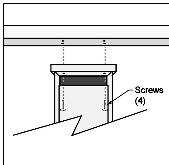
FIGURE 2-8. T107 Sensor Arm Mounting
