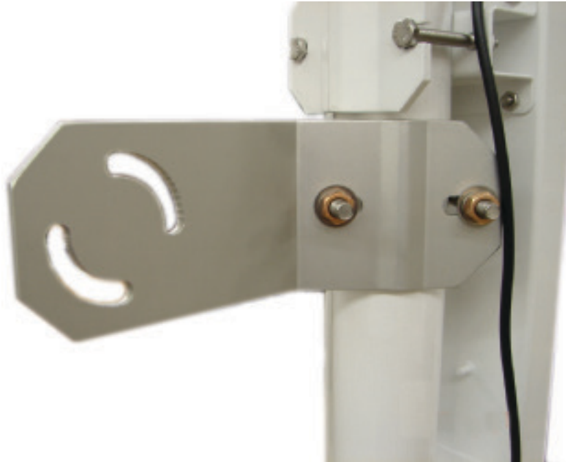
FIGURE 2-32. Antenna Bracket Mounted to Pole
