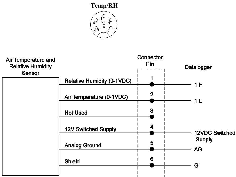
FIGURE 4-3. Schematic of HMP60-ETS RH and Temperature Probe and Connector Temp/RH
