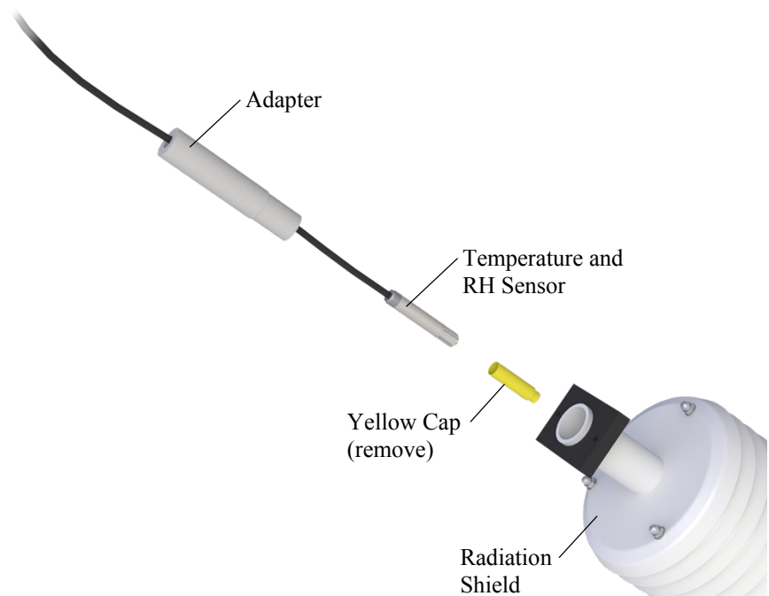
FIGURE 2-9. Temperature/Relative Humidity Sensor with Yellow Protective Cap
