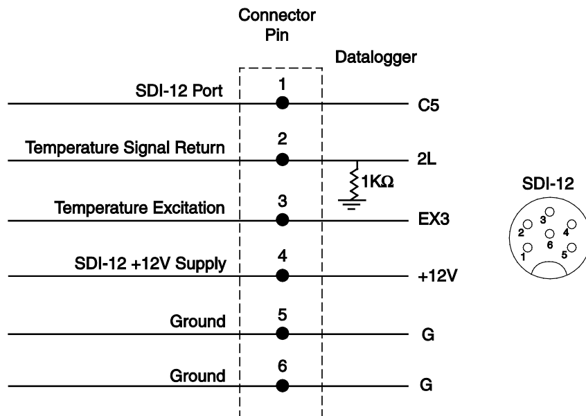
FIGURE 4-9. Schematic of Connector SDI-12
