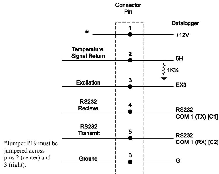
FIGURE 4-5. Schematic of Gill WindSonic1-ET Wind Sensor, Soil Temperature Sensor (107-LC or 108-LC), and Connector Temp/Sonic
