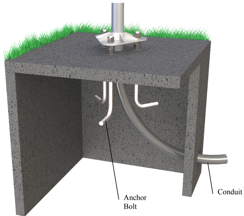
FIGURE 2-3. Cut-Away View Shows Anchor Bolt and Conduit Placement in Cement Pad
