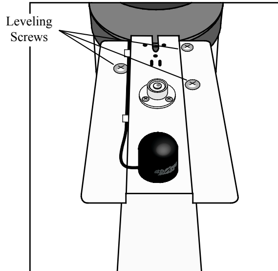
FIGURE 2-19. Pyranometer Leveling
