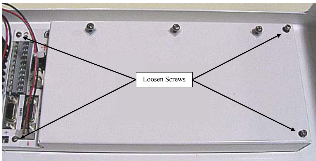
FIGURE 2-13. Screws that Secure the Electronics Cover
