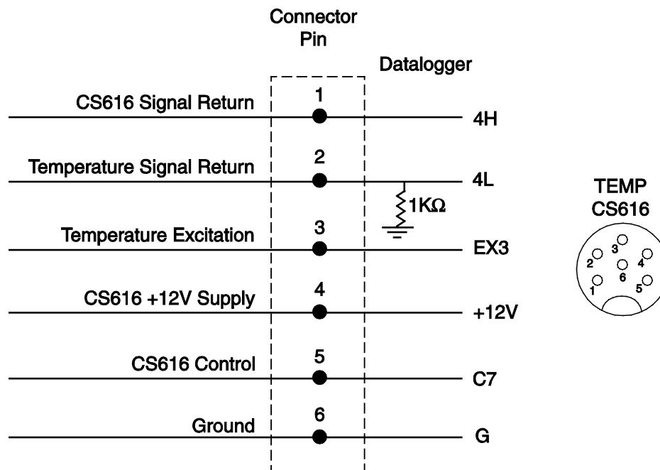
FIGURE 4-8. Schematic of 107-LC or 108-LC Temperature Probe or CS616-LC Soil Volumetric Water Content Sensor and Connector Temp/CS616
