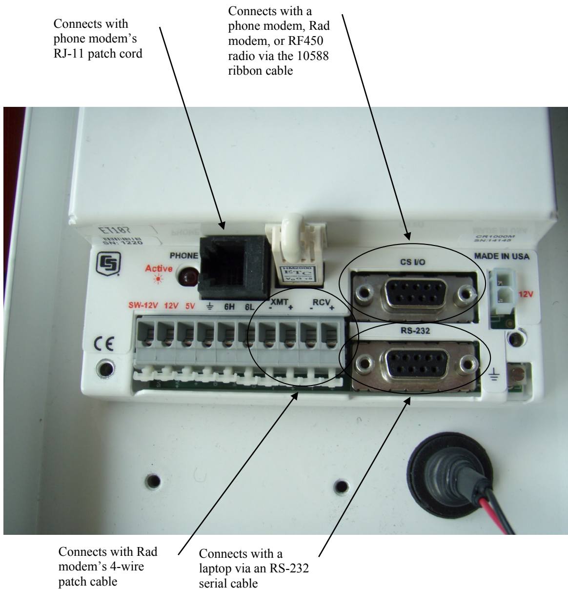
FIGURE 2-23. Close-up of the terminals and 9-pin ports in the T107 (battery not shown).
