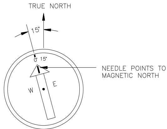
FIGURE 1-8. Declination Angles West of True North Are Added to 0 to Get True North
