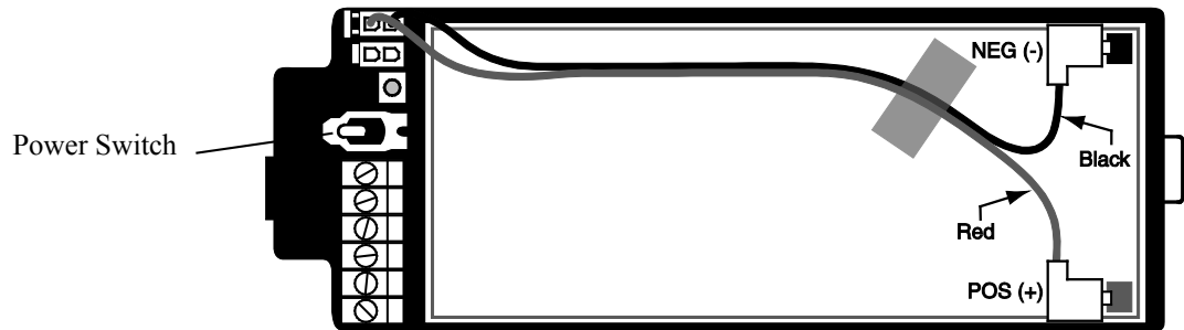
FIGURE 2-43. PS100 Battery Installation
