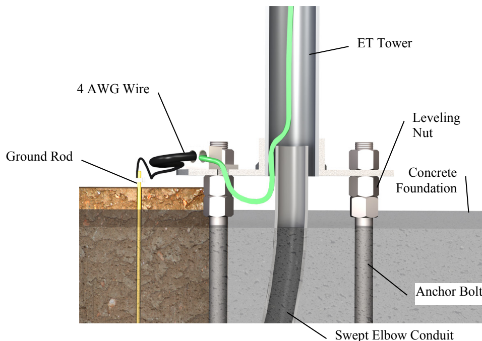
FIGURE 2-4. Transparent View Shows Raising and Grounding the ET Tower
