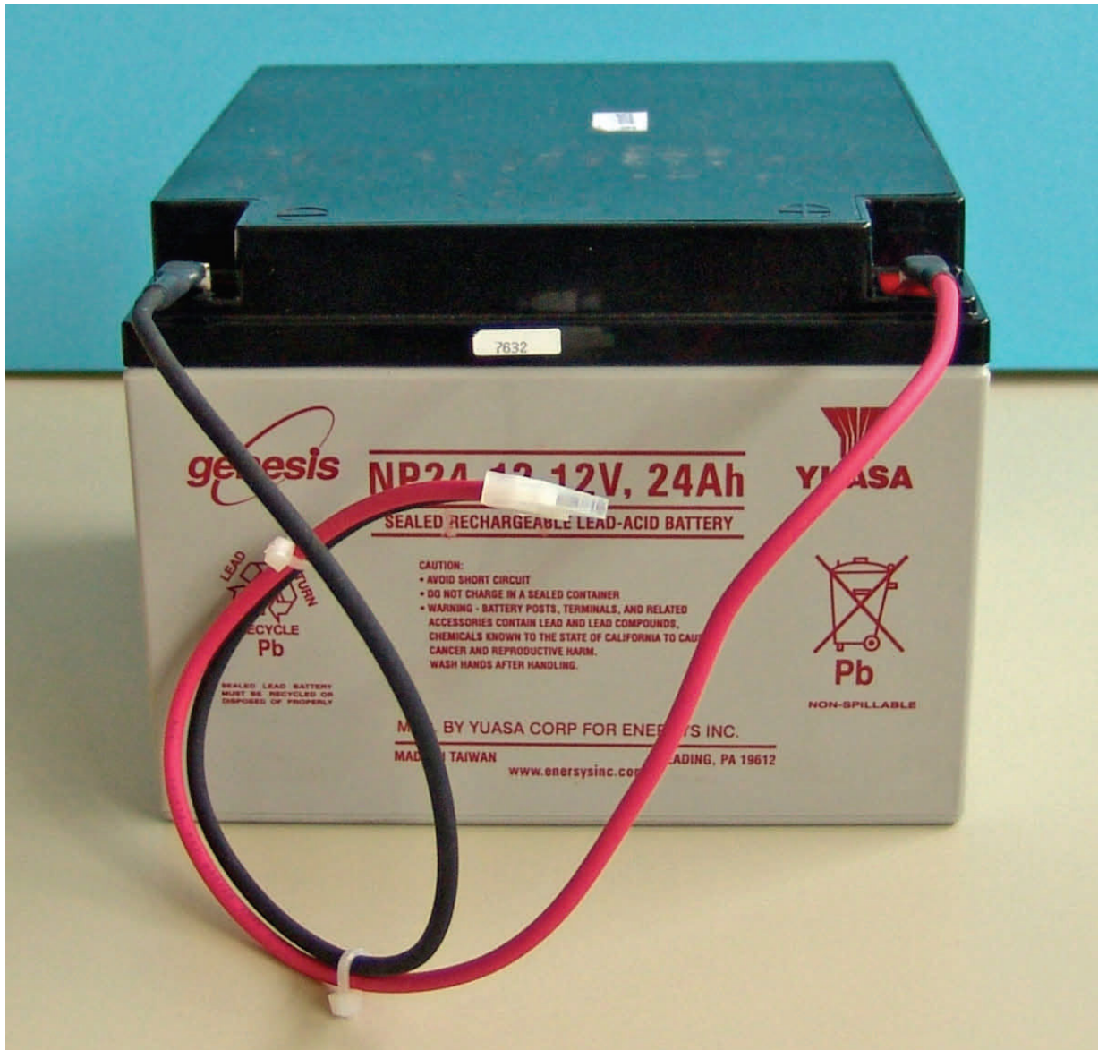
FIGURE B-2. 24 Ahr Battery and Battery Cable
