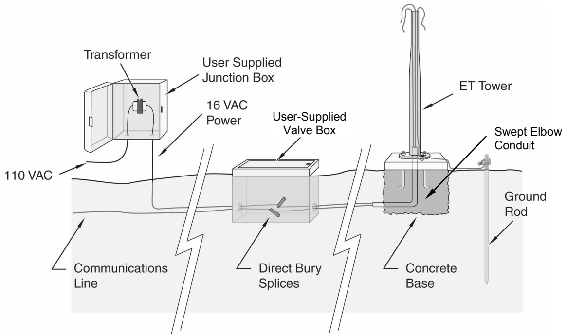
FIGURE E-1. ET tower installation with step-down transformer
