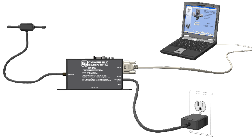
FIGURE 2-37. Base RF450 Installation
