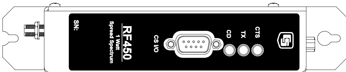
FIGURE 4-2. RF450 Front Side View
