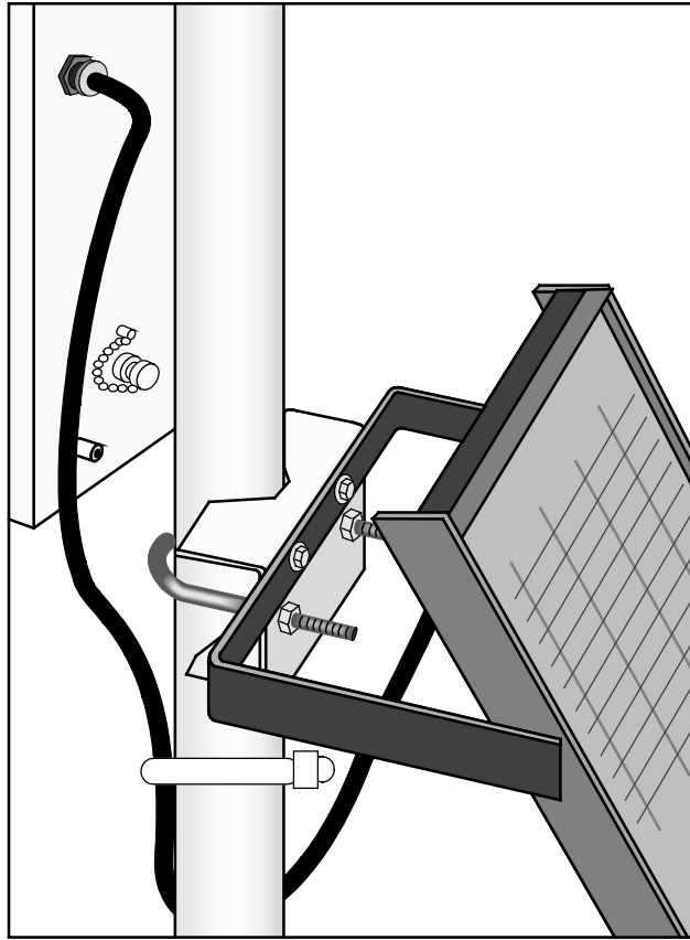
FIGURE 2-41. Solar Panel Mounting and Cabling
