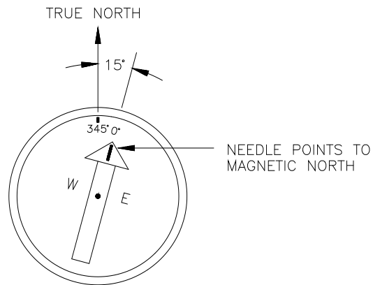
FIGURE 1-7. Declination Angles East of True North Are Subtracted From 0 to Get True North
