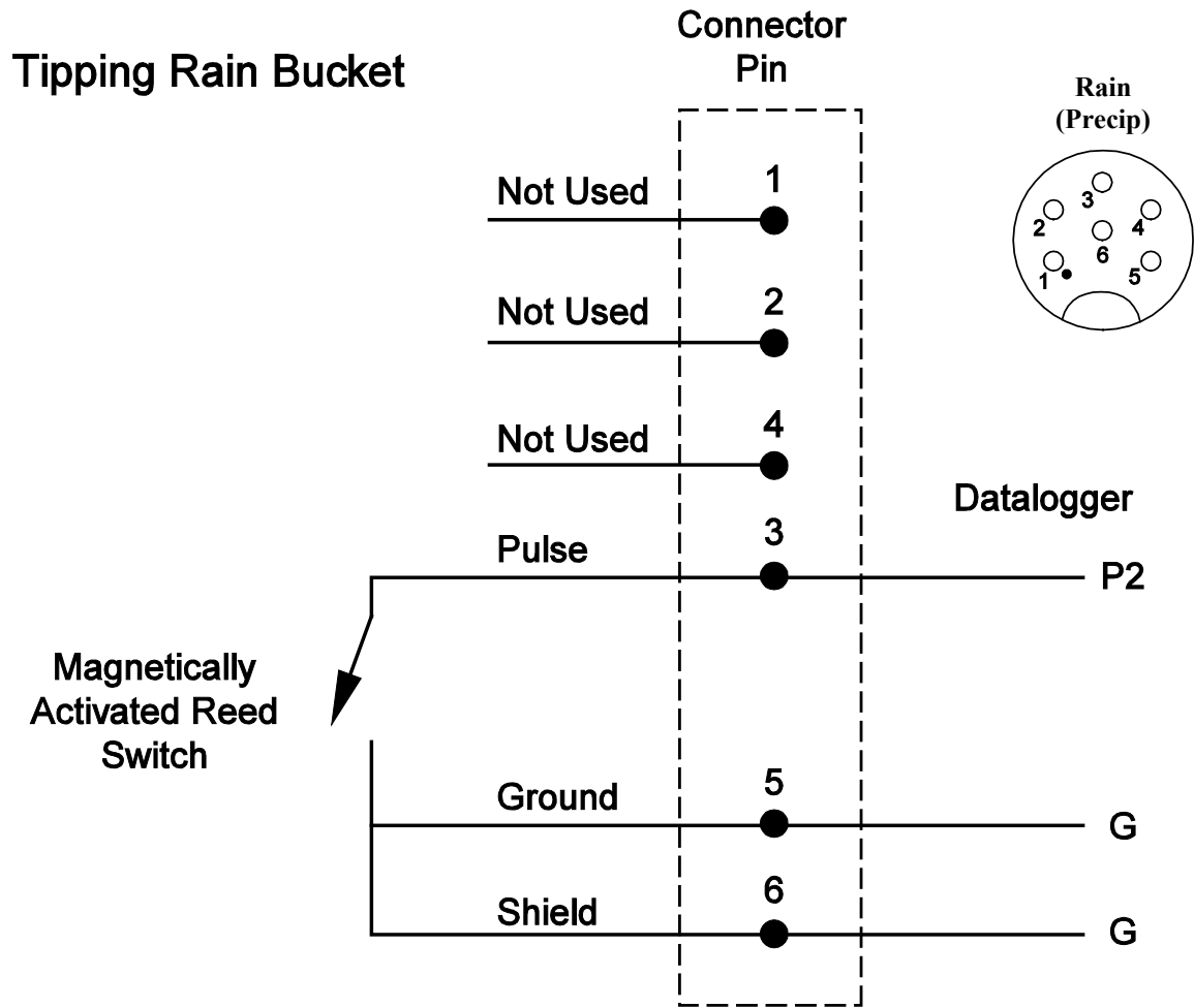
FIGURE 4-7. Schematic of TE525-ET Rain Sensor and Connector Rain (Precip)
