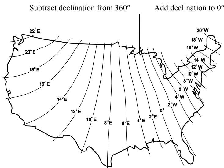
FIGURE 1-6. Magnetic Declination for the Contiguous United States
