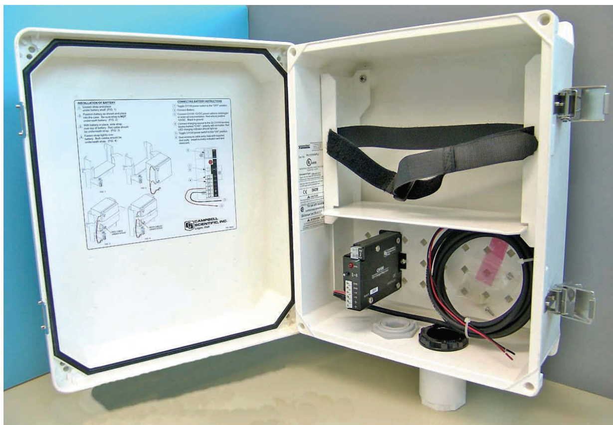
FIGURE B-1. Environmental Enclosure with CH100, Power Cable, and Battery Bracket
