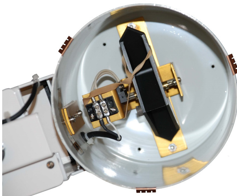
FIGURE 2-18. Remove Rubber Band from Tipping Mechanism
