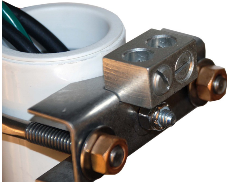
FIGURE 2-39. Lightning Rod Bracket Installation
