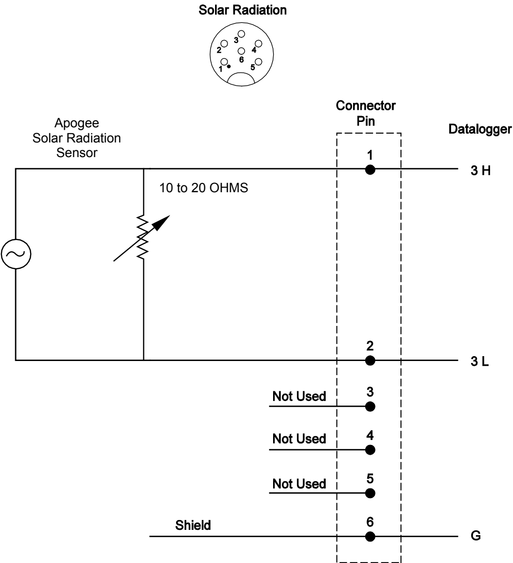
FIGURE 4-6. Schematic of CS305-ET Solar Radiation Sensor and Connector Solar Radiation
