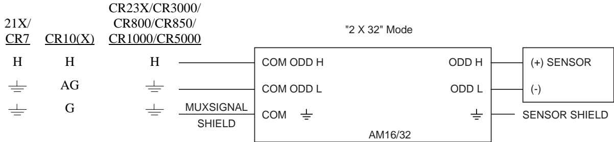
FIGURE 10. Single-ended Measurement without Excitation
