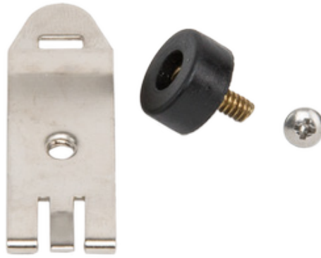
FIGURE 7-4. CDM DIN-Rail Mounting Kit
