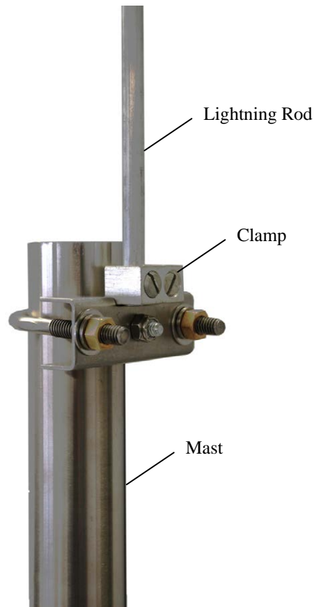
FIGURE 5-9. Lightning rod and tripod ground lug
