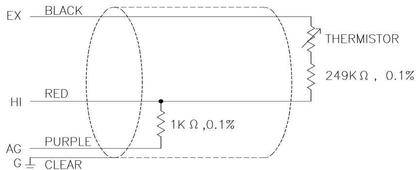
FIGURE 6-3. 107 Thermistor Probe Schematic
