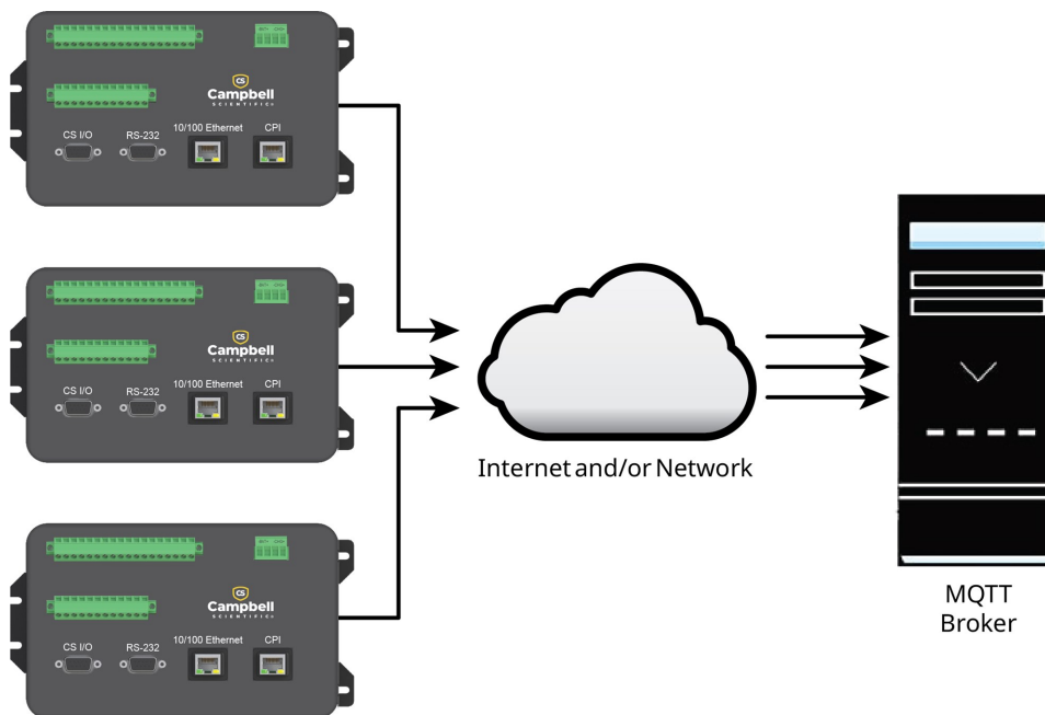
Figure 10-11. Transmitting data (JSON) from data loggers to a server.
