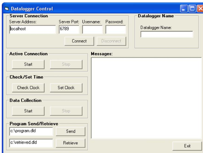
FIGURE 9-1. CsiDatalogger Example
