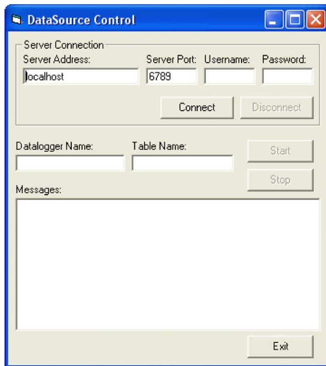
FIGURE 11-1. CsiDataSource Example
