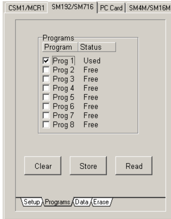
FIGURE 10.4-1. PROGRAMS Screen
