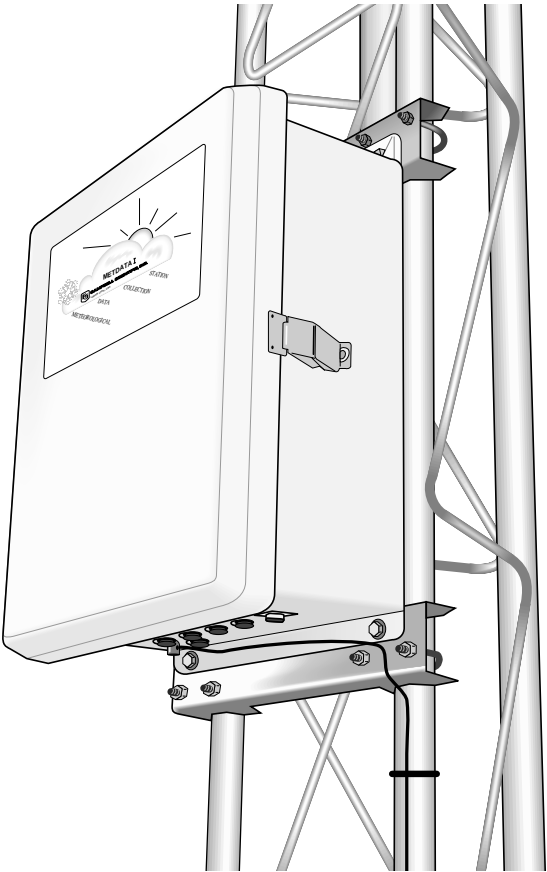
FIGURE 3.1-2. MetData1 Enclosure on UT10 or UT30 Tower
