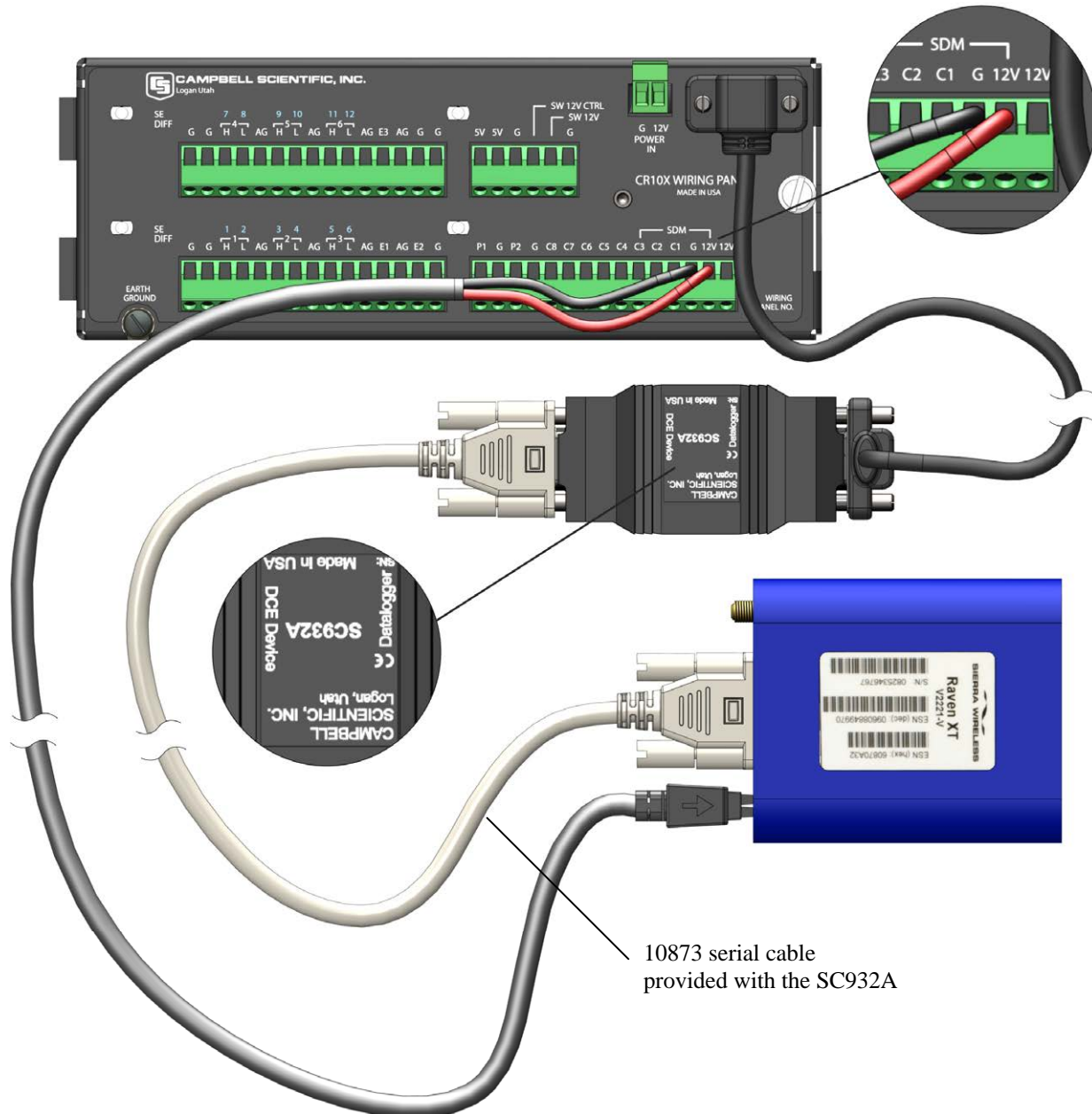
FIGURE 4-4. Connections using the SC932A
